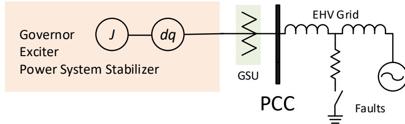
Figure 4: Rotating machine plant model components connected to a SMIB test system [17]
