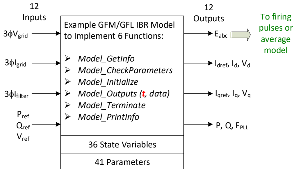
Figure 6: DLL interface for example IBR control code models of grid-forming (GFM) and grid-following (GFL) inverters [17]
