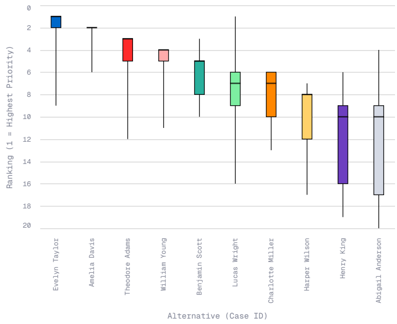
B) Ranks Box Plot
