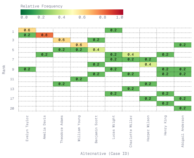
C) Rank Acceptability Indices
