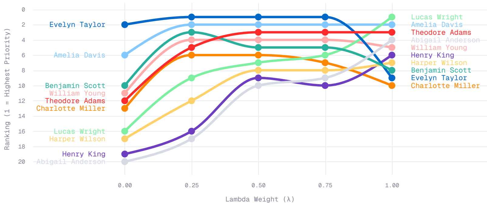
A) Bump Chart
