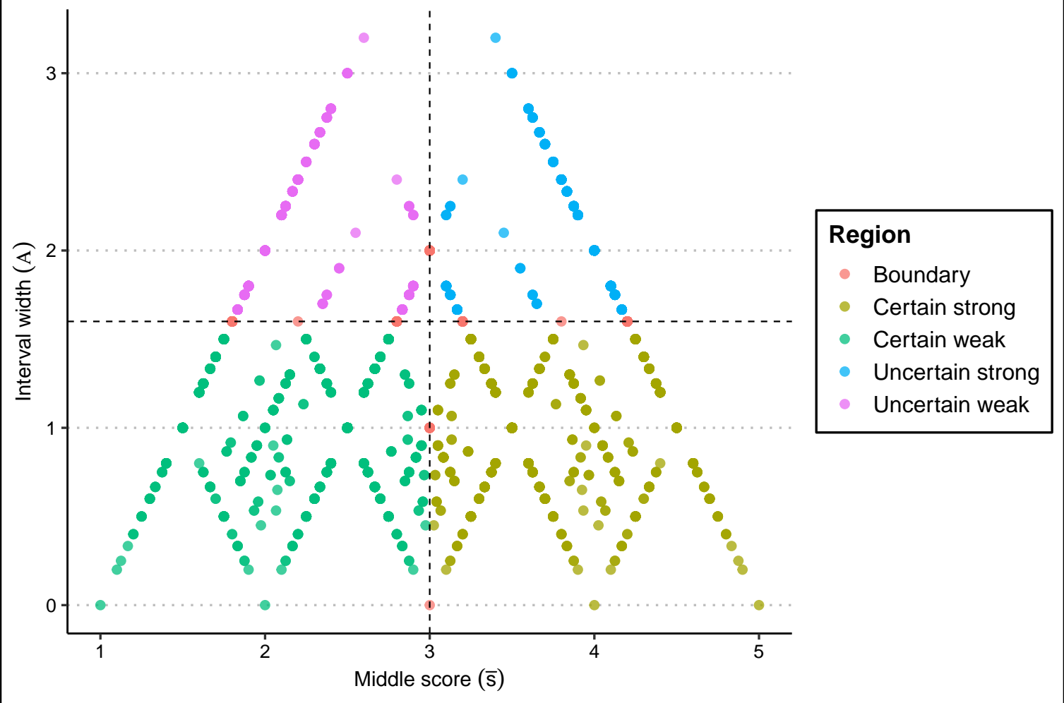
Discrete performance landscape (conservative view)
