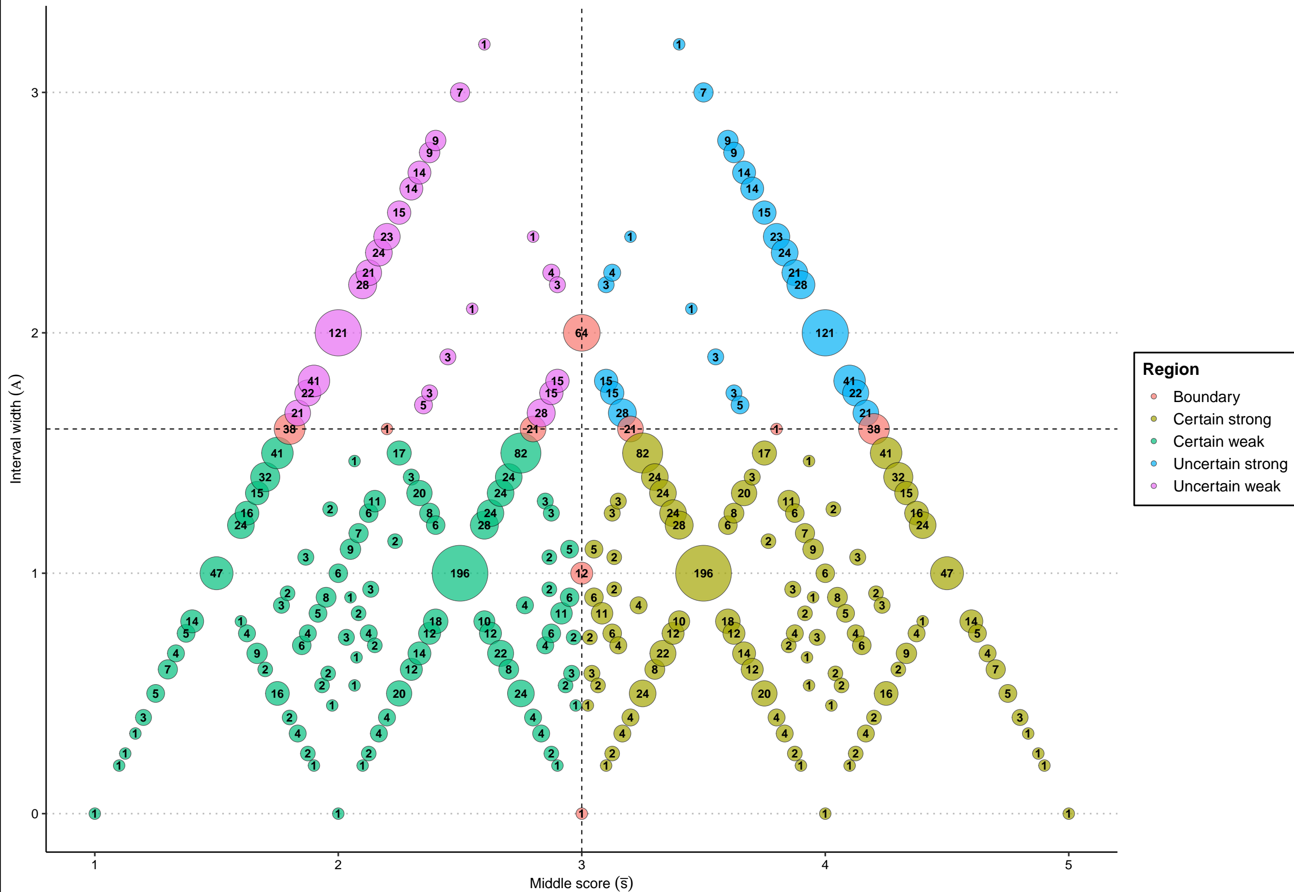
Discrete performance landscape (bubble, n = 5 )
