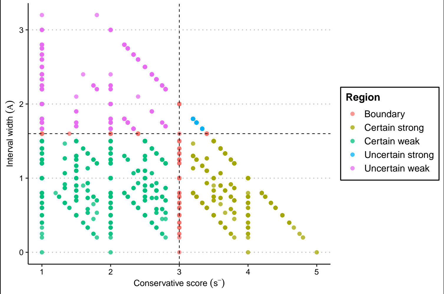
Discrete performance landscape (optimistic view)
