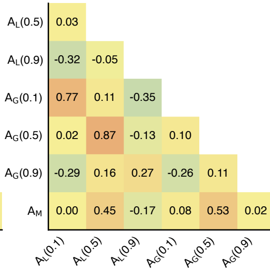
(e) Jaccard, \sigma_R = 0.10
