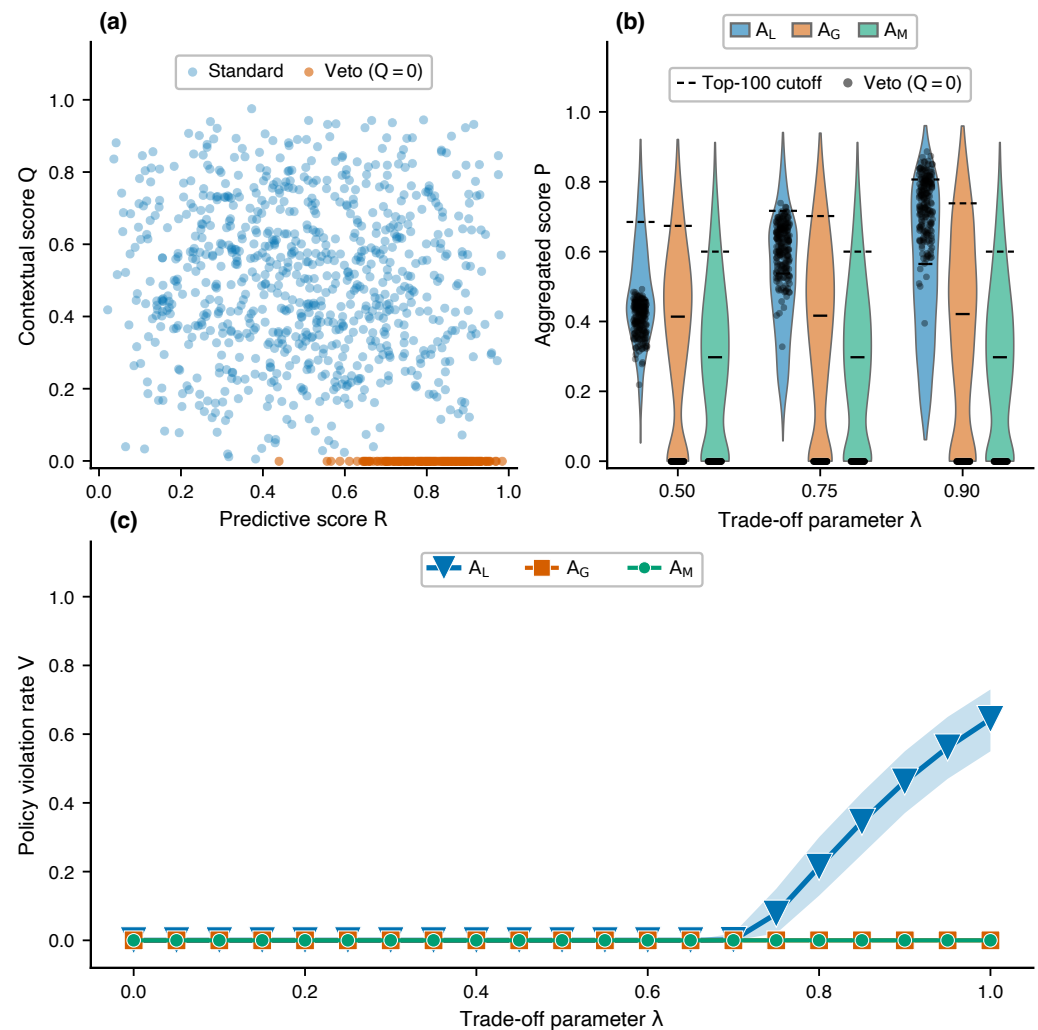
Figure 1. Policy compliance under contextual vetoes ( N = 1000 , K = 100 ). The veto group (20% of cases) has Q_i = 0 and high predictive scores, creating adversarial conflict between prediction and context. (a) Illustrative synthetic population (Monte Carlo trial 0): scatter of R_i versus Q_i ; standard cases and contextual vetoes are shown separately. (b) For the same population, violin distributions of the aggregated scores P_i for A_L , A_G , and A_M at \lambda \in \{0.50, 0.75, 0.90\} . Dashed horizontal segments indicate the Top- K score threshold, while jittered points identify vetoed alternatives ( Q_i = 0 ). Their position relative to the threshold shows directly whether vetoed alternatives can enter the selected set. (c) Monte Carlo mean policy violation rate V(\lambda) over 1000 replications for the dense sweep \lambda \in [0, 1] ; shaded bands denote 95% percentile intervals.
