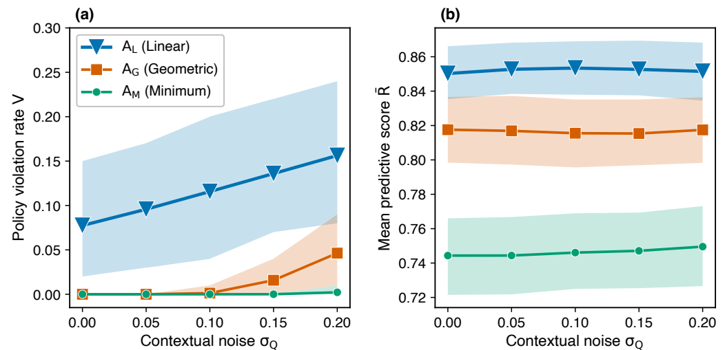
Figure 3. Sensitivity to contextual noise at \lambda = 0.75 . Contextual scores are perturbed as Q'_i = \text{clip}(Q_i + \epsilon_i, 0, 1) , \epsilon_i \sim \mathcal{N}(0, \sigma_Q^2) ; aggregation uses Q'_i while policy violations are evaluated using the true Q_i . Results are Monte Carlo means with 95% percentile intervals over 1000 replications ( N = 1000 , K = 100 ). (a) Policy violation rate V(\sigma_Q) . (b) Mean original predictive score \bar{R}(\sigma_Q) .
