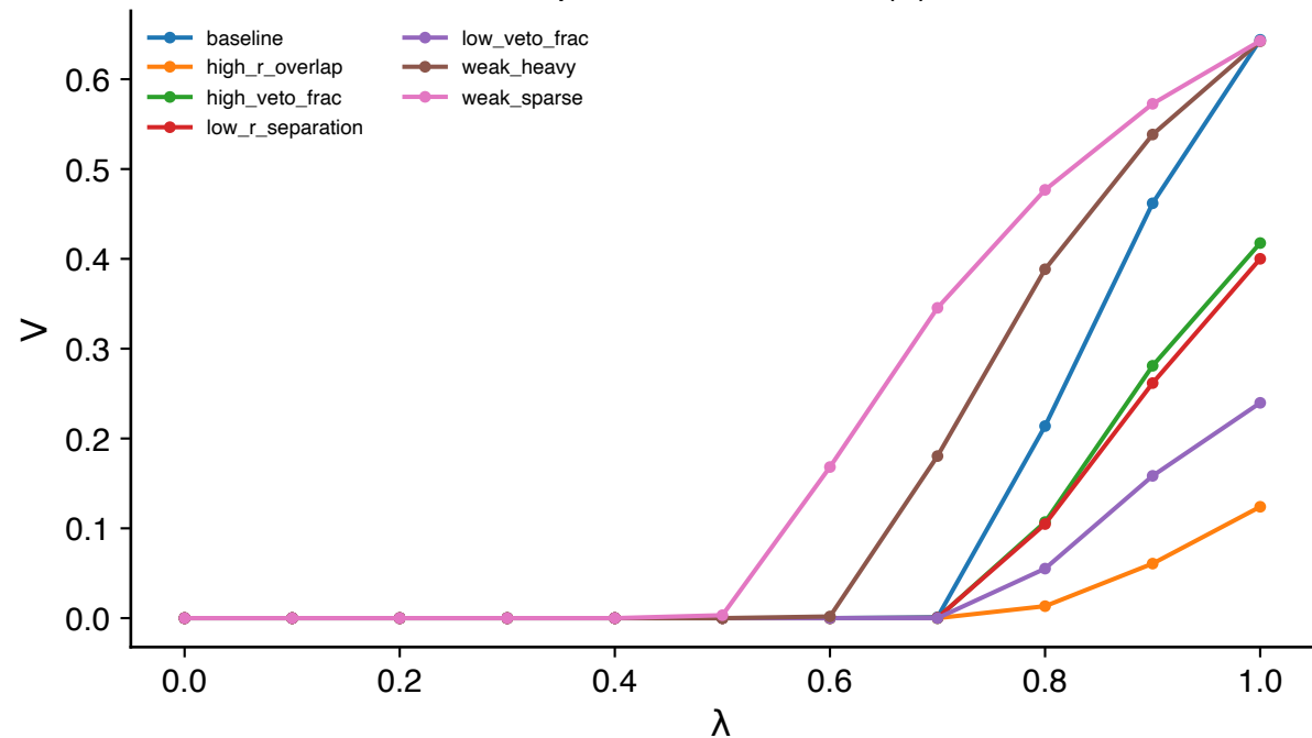
Population variants: V(\lambda)
