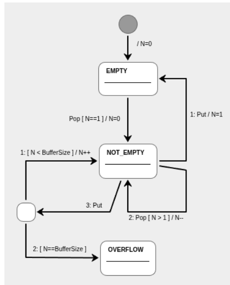
Fig. 16: State Machine for a Buffer Control Logic
