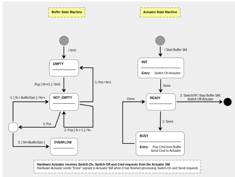
Fig. 18: State Machines to Control the Hardware Actuator
