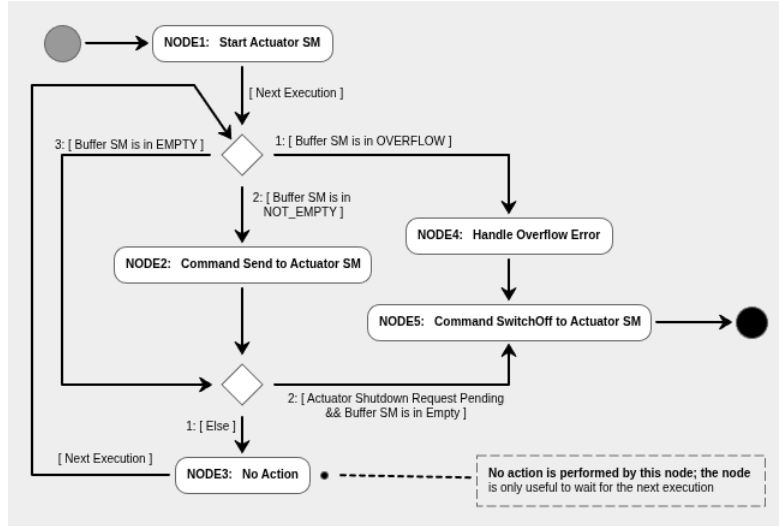
Fig. 17: Procedure to Control a Hardware Actuator
