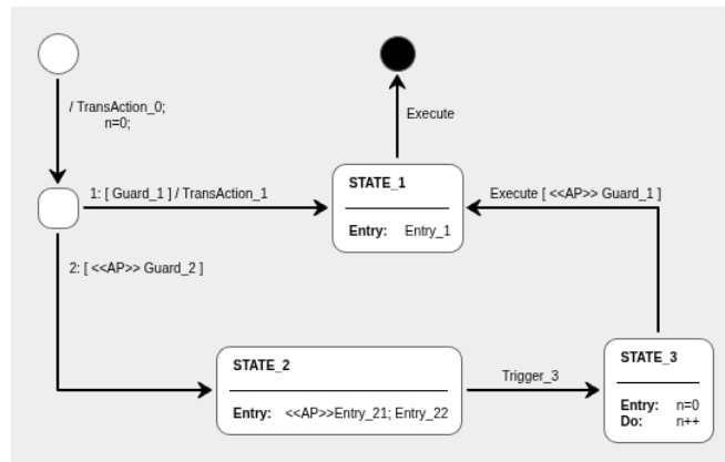
Fig. 9: Example of FW-Compliant State Machine
