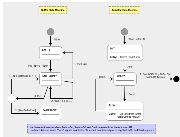
Fig. 18: State Machines to Control the Hardware Actuator
