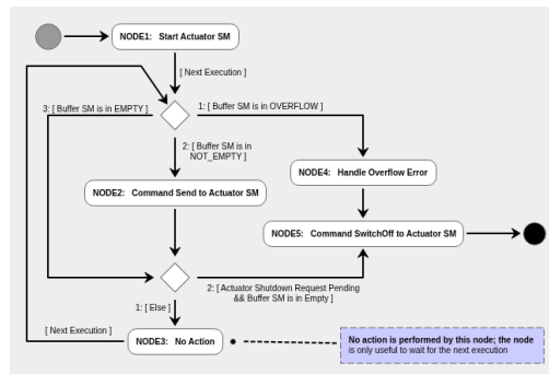
Fig. 17: Procedure to Control a Hardware Actuator
