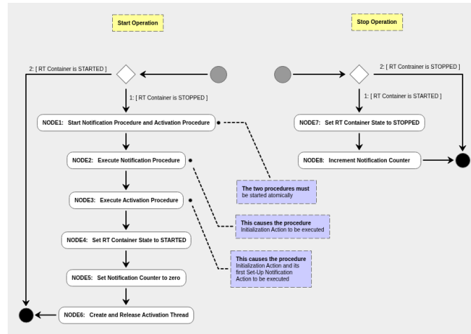
Fig. 12: Start and Stop Operations for RT Containers
