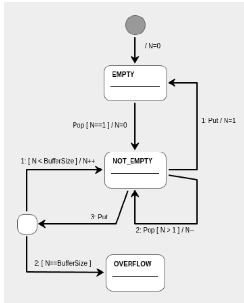
Fig. 16: State Machine for a Buffer Control Logic
