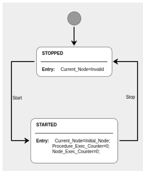
Fig. 3: Procedure Start/Stop Commands
