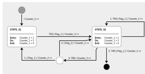
Fig. 4: Test State Machine SM5
