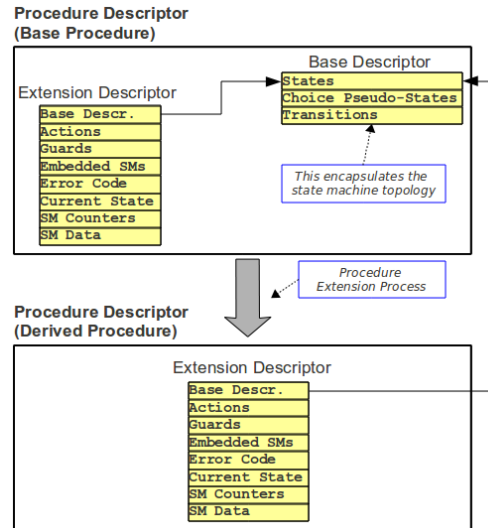
Fig. 7: Extension Mechanism for Procedure Descriptors
