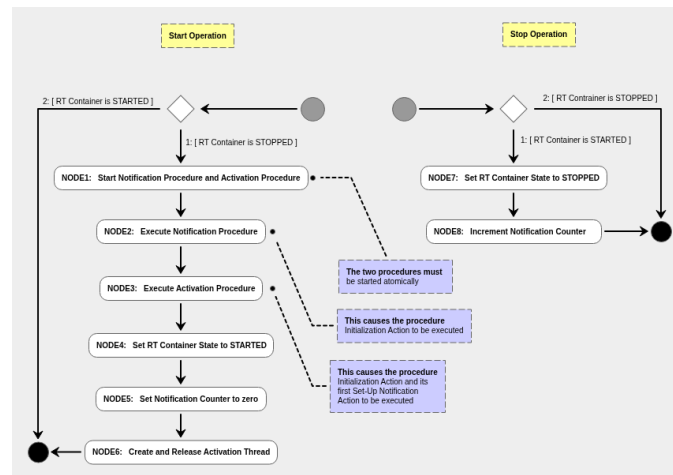
Fig. 13: Start and Stop Operations for RT Containers
