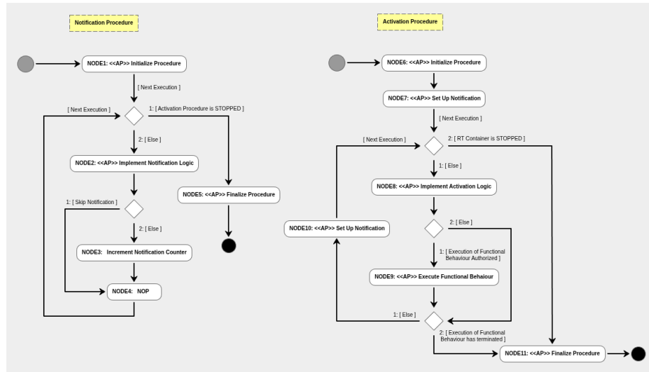
Fig. 14: RT Container Procedures
