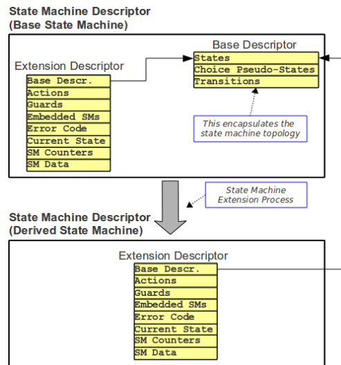
Fig. 5: Extension Mechanism for State Machine Descriptors
