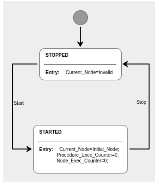
Fig. 11: Procedure Start/Stop Commands
