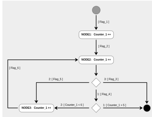
Fig. 6: Test procedure PR2
