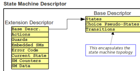
Fig. 1: Internal Structure of a State Machine Descriptor
