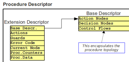
Fig. 2: Internal Structure of a Procedure Descriptor
