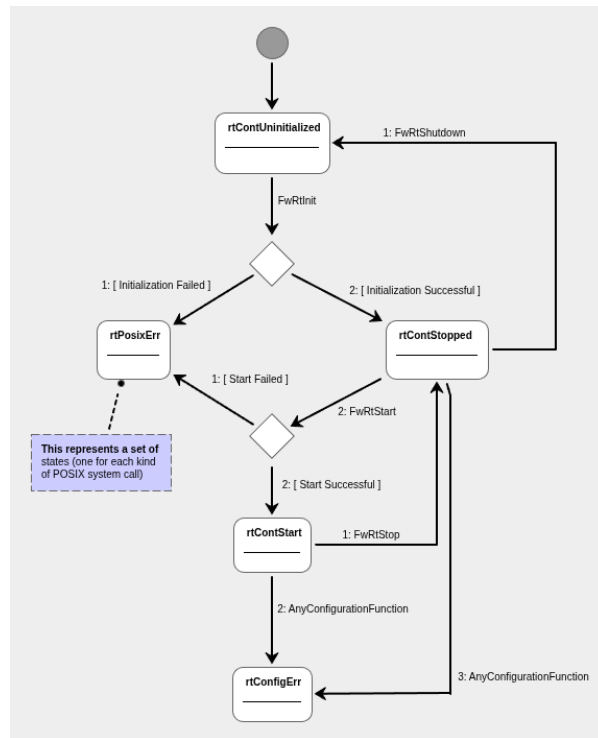
Fig. 3: RT Container States
