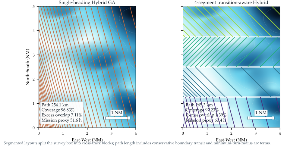
Figure 8. Gate-aware blockwise fixed-line repair for the synthetic Complex Terrain failure case for the MBES numerical benchmark. The accepted four-segment layout restores the C97/O3 gate while accounting for inter-block transits, heading changes, and line-change arcs. This is a numerical blockwise-layout extension, not a vehicle-dynamics model or executed-survey record.
