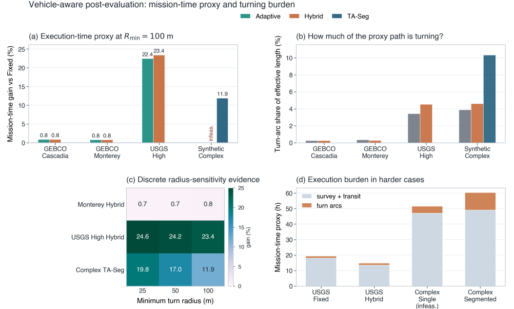
Figure 5. Vehicle-aware post-evaluation for the MBES public-grid numerical benchmark using a minimum-turn-radius and mission-time proxy. The diagnostic adds semicircular line-change arcs to the reported line families and converts distance into time with declared survey and turn speeds. Infeasible layouts are marked rather than promoted as valid gains; the figure reports an execution-boundary stress check, not a current-aware controller simulation or mission record.
