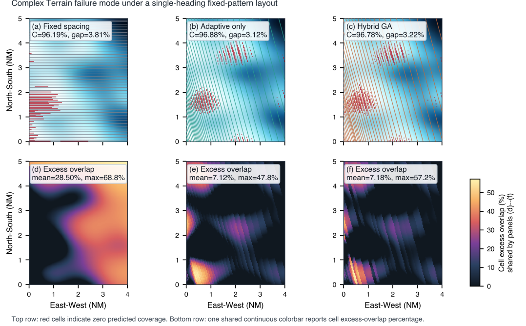
Figure 7. Failure-mode visualization for the synthetic-grid MBES numerical benchmark. Panels (a)–(c) mark zero-predicted-coverage cells on the planned line families, and panels (d)–(f) show the corresponding cellwise excess-overlap fields. The figure explains why global fixed-heading methods can fail even after local refinement and motivates a constrained blockwise repair without introducing a realized-operation case.
