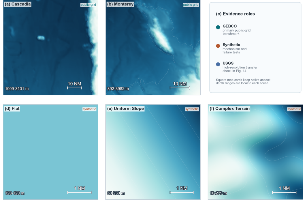
Figure 2. Benchmark atlas for the five terrains used in this study. Panels (a)–(b) are public GEBCO 2025 bathymetry subsets, panel (c) states evidence roles, and panels (d)–(f) are synthetic mechanism tests. Cards preserve scene-specific extents and depth ranges; they support a public-grid numerical benchmark, not evidence from an executed survey.
