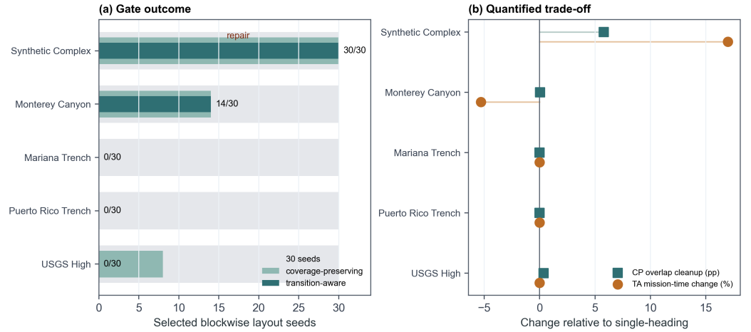
Figure 9. Decision audit for the gate-aware blockwise fixed-line extension, recomputed from segmented_heading_extension/segmented_heading_raw for the MBES numerical benchmark.csv. Panel (a) counts accepted blockwise seeds under coverage-preserving and transition-aware selectors; panel (b) reports overlap cleanup and mission-time trade-offs relative to single-heading Hybrid GA. The audit documents mandatory repair on synthetic Complex Terrain, selective acceptance on Monterey Canyon, and rejection when coverage loss or transition burden outweighs cleanup.
