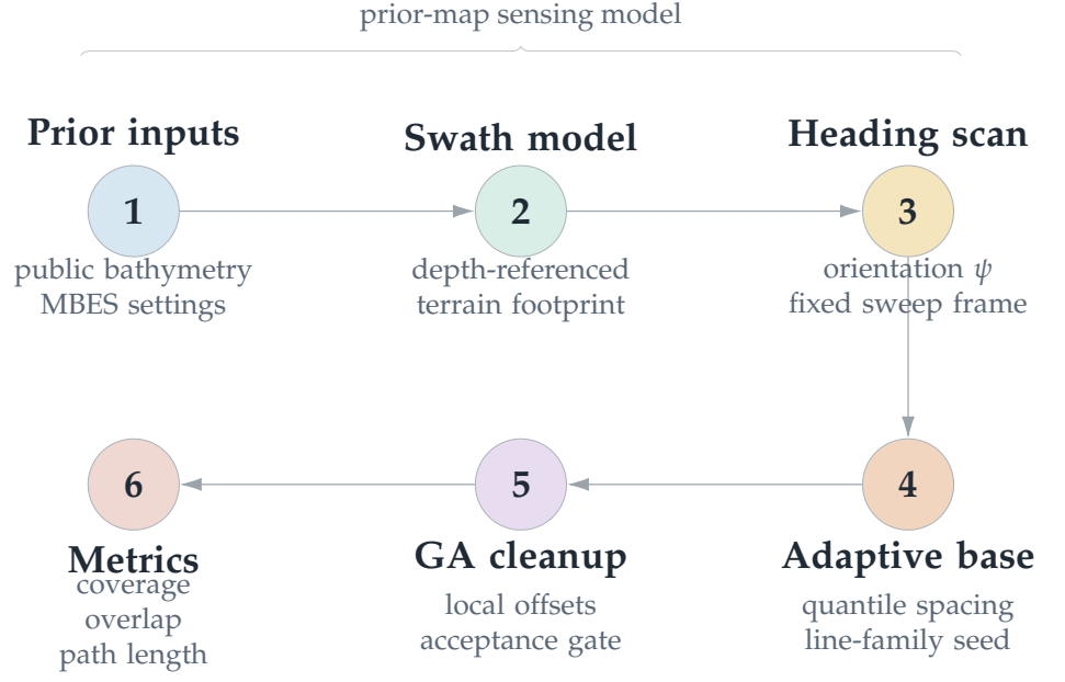
Figure 1. Workflow of the fixed-line MBES planning benchmark. A prior bathymetric grid and MBES settings define terrain-dependent swath estimates; a heading scan selects \psi ; adaptive spacing, optional local GA refinement, and gate-aware blockwise repair place the line family; and the evaluator reports path length, predicted coverage, excess overlap, feasibility, and seed repeatability.
