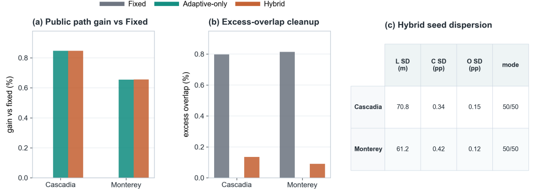
Figure 12. Public-scene ablation and seed-level dispersion from the reported MBES numerical benchmark. Panels (a) and (b) compare Fixed-Spacing, Adaptive Spacing without GA, and Full Geometry-Aware Hybrid GA on path gain relative to Fixed-Spacing and on excess-overlap violation for the two public GEBCO scenes. Panel (c) reports the standard deviation of Hybrid GA path length L , predicted coverage C , and excess overlap O across 50 seeds, together with the count of seeds that converged to the dominant orientation/line-count mode.
