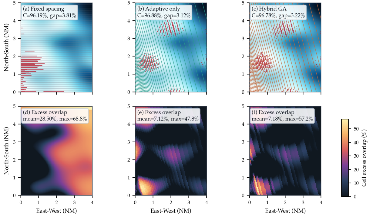
Complex Terrain failure mode under a single-heading fixed-pattern layout
