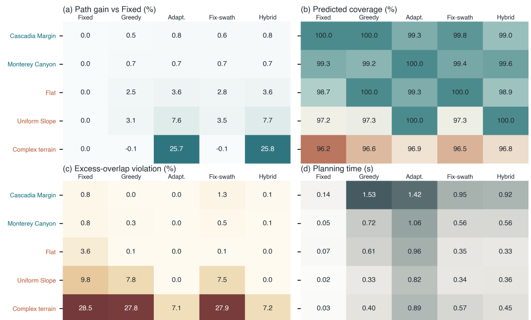
Figure 9. Cross-scene metric matrix from the reported benchmark. Each panel is a scene-by-method heatmap of benchmark means: path gain relative to Fixed-Spacing, predicted coverage, excess-overlap violation, and planning time. The top two rows are the public GEBCO scenes and the bottom three rows are synthetic stress tests, so the figure exposes both the public-data pattern and the complex-terrain failure boundary in one compact view. Stochastic GA methods report 50-seed means, and all coverage values are numerical predictions rather than field measurements.
