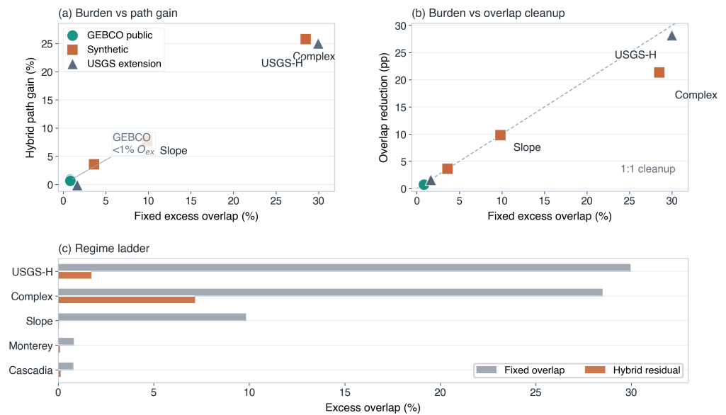
Figure 10. Scene-level regime diagnostic linking the Fixed-Swath baseline to the observed Hybrid benefit. Each point is one scene from either the reported main benchmark or the separate USGS 30 m extension. Panel (a) plots Fixed-Swath excess-overlap burden against Hybrid path gain relative to Fixed-Swath. Panel (b) plots the same burden against Hybrid overlap reduction. Panel (c) gives a ranked overlap-regime ladder, comparing the Fixed-Swath burden with the Hybrid residual on representative scenes. The GEBCO public scenes cluster in a low-overlap regime below 1 percent excess overlap, whereas Complex Terrain and the high-complexity USGS crop start near 30 percent excess overlap and therefore show the largest geometry-aware gains. The USGS points strengthen the mechanism interpretation but are not merged into the main benchmark averages reported elsewhere in the paper.
