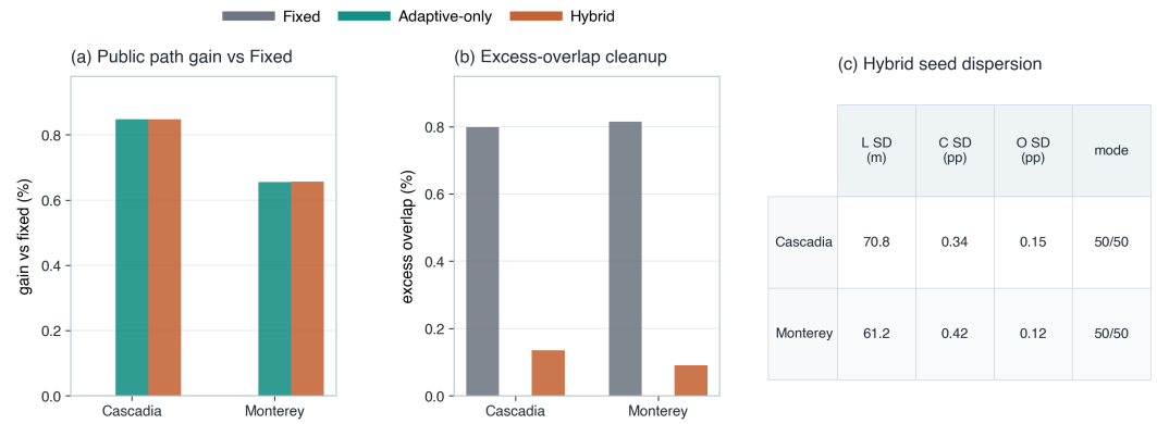
Figure 11. Public-scene ablation and seed-level dispersion from the reported benchmark. Panels (a) and (b) compare Fixed-Spacing, Adaptive Spacing without GA, and Full Geometry-Aware Hybrid GA on path gain relative to Fixed-Spacing and on excess-overlap violation for the two public GEBCO scenes. Panel (c) reports the standard deviation of Hybrid GA path length L , predicted coverage C , and excess overlap O across 50 seeds, together with the count of seeds that converged to the dominant orientation/line-count mode.
