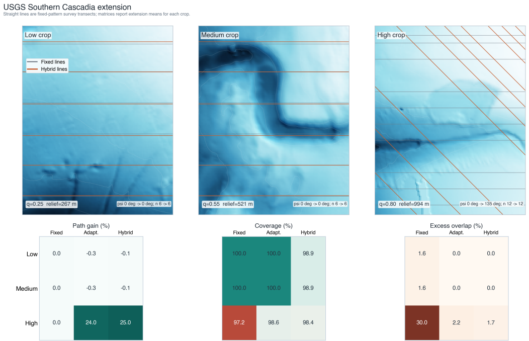
Figure 15. Independent USGS Southern Cascadia 30 m multibeam-derived public-grid extension. The top row shows the three selected crops with Fixed-Spacing and representative Hybrid GA line families, ordered by empirical terrain complexity from low to high and drawn without map-axis distortion. The bottom row reports benchmark means for path gain relative to Fixed-Spacing, predicted coverage, and excess-overlap violation recomputed from the extension CSV/JSON outputs. These plotted straight transects are planned fixed-pattern survey-line families, not free-form vehicle trajectories. The extension remains a public-grid numerical check, not an additional sea-trial or mission-log validation.
