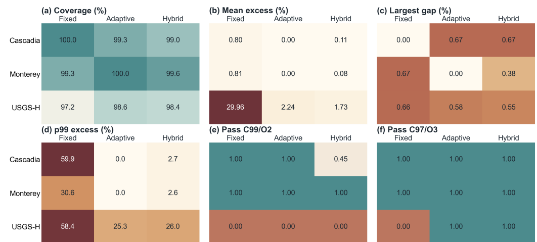
Figure 16. Threshold and local-failure diagnostic for the two primary GEBCO scenes and the USGS high-complexity crop. The figure reports mean coverage, mean excess-overlap violation, largest connected uncovered patch, the 99th-percentile cellwise excess-overlap tail, and pass rates under both the stricter C99/O2 screen and the manuscript's default C97/O3 benchmark gate. Hybrid GA values are 20-seed means; Fixed-Spacing and Adaptive Spacing without GA are deterministic. The diagnostic is a raster-evaluator audit designed to expose local failures hidden by scene-level means; it is not hydrographic QA or a field-survey acceptance test.
