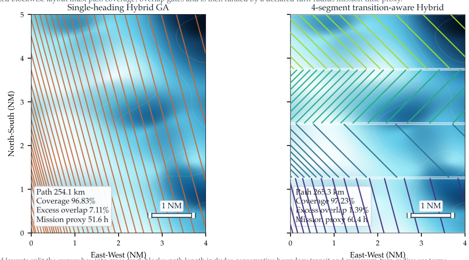
Figure 7. Gate-aware blockwise fixed-line repair for the synthetic Complex Terrain failure case. The left panel shows a representative single-heading Hybrid GA layout, which is faster under the declared mission-time proxy but remains infeasible because predicted coverage stays below the 97 percent threshold and excess overlap remains above the reported acceptance margin. The right panel shows the accepted four-segment Hybrid GA extension, where each block selects its own heading and spacing margin while the reported path length and selector include conservative inter-block transits, minimum-turn-radius heading-change terms, and line-change turn arcs. This figure is a numerical blockwise-layout extension, not a sea-trial or vehicle-dynamics validation.
