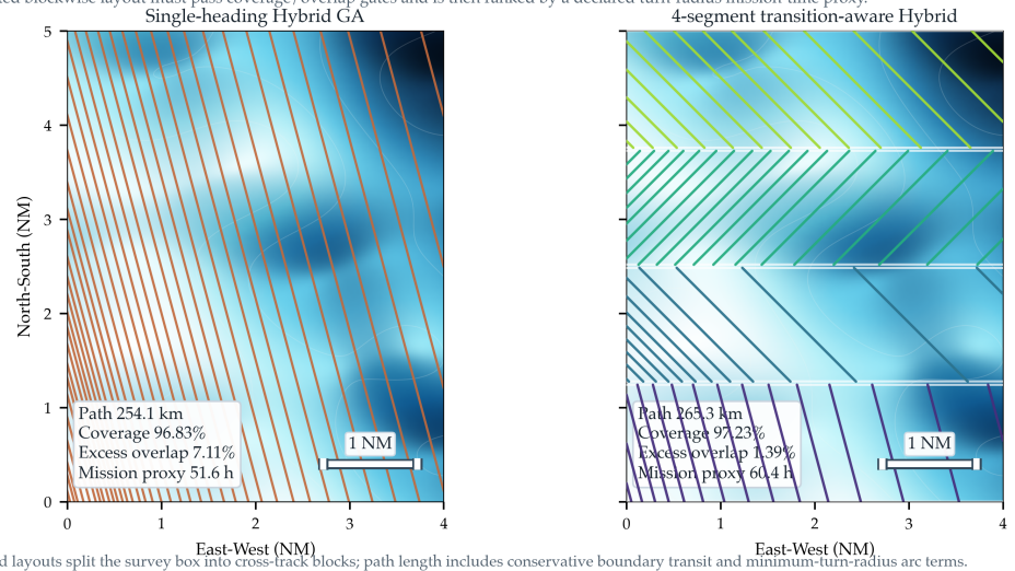
Figure 7. Transition-aware segmented-heading repair diagnostic for the synthetic Complex Terrain failure case. The left panel shows a representative single-heading Hybrid GA layout, which is faster under the declared mission-time proxy but remains infeasible because predicted coverage stays below the 97 percent threshold and excess overlap remains above the reported acceptance margin. The right panel shows the accepted four-segment Hybrid GA extension, where each block selects its own heading and spacing margin while the reported path length and selector include conservative inter-block transits, minimum-turn-radius heading-change terms, and line-change turn arcs. This figure is a numerical blockwise-layout diagnostic, not a sea-trial or vehicle-dynamics validation.
