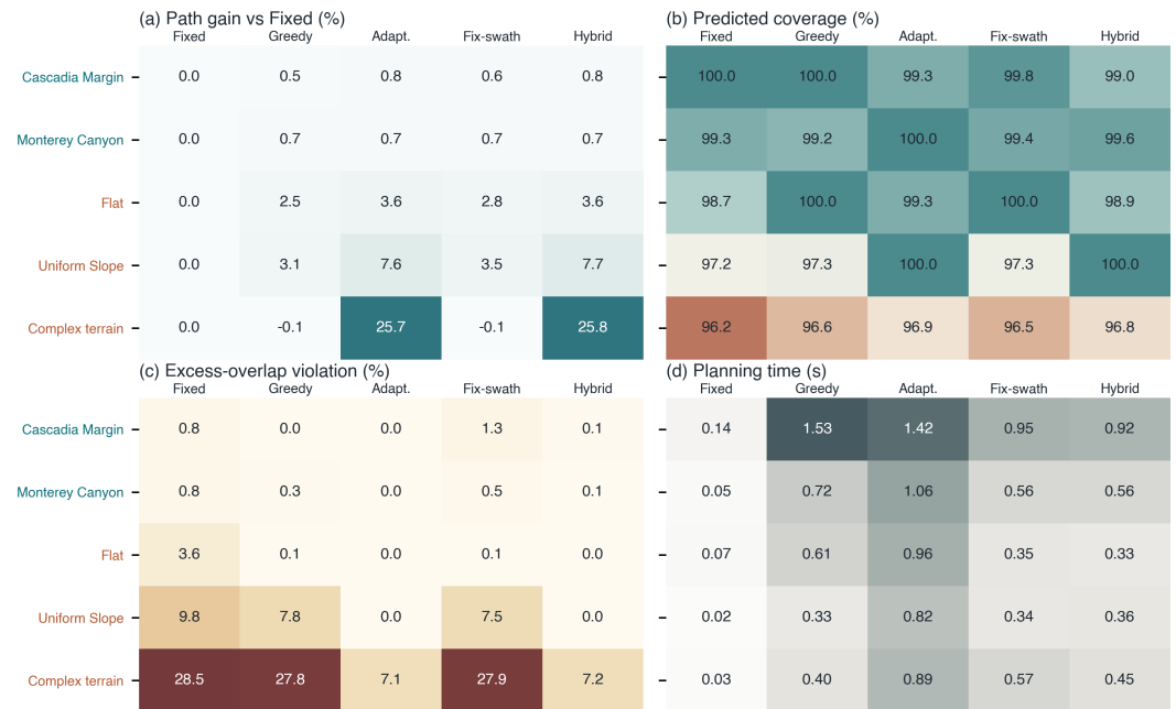
Figure 8. Cross-scene metric matrix from the reported benchmark. Each panel is a scene-by-method heatmap of benchmark means: path gain relative to Fixed-Spacing, predicted coverage, excess-overlap violation, and planning time. The top two rows are the public GEBCO scenes and the bottom three rows are synthetic stress tests, so the figure exposes both the public-data pattern and the complex-terrain failure boundary in one compact view. Stochastic GA methods report 50-seed means, and all coverage values are numerical predictions rather than field measurements.
