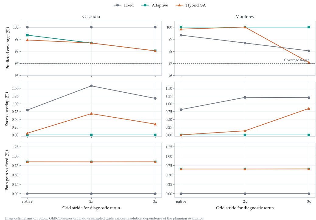
Figure 10. Public-scene grid-resolution sensitivity diagnostic. The same three public-scene methods are rerun on the native GEBCO-derived grids and on 2\times and 3\times strided downsampled grids using the reported evaluator. Hybrid GA reports seeds 0–4 for this diagnostic, whereas the main benchmark remains the native-grid 20-seed benchmark used in this study. The Monterey 3\times case exposes a resolution-dependent coverage boundary for the Hybrid GA, so the diagnostic should be interpreted as a planning-evaluator sensitivity check rather than as field-performance evidence.
