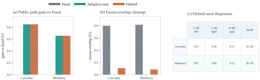
Figure 7. Public-scene ablation and seed-level dispersion from the reported benchmark. Panels (a) and (b) compare Fixed-Spacing, Adaptive Spacing without GA, and Full Geometry-Aware Hybrid GA on path gain relative to Fixed-Spacing and on excess-overlap violation for the two public GEBCO scenes. Panel (c) reports the standard deviation of Hybrid GA path length L , predicted coverage C , and excess overlap O across 20 seeds, together with the count of seeds that converged to the dominant orientation/line-count mode.
