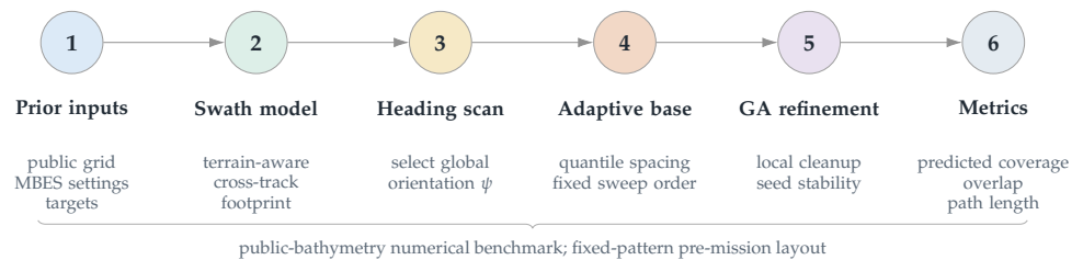
Figure 1. Method workflow for the proposed terrain-aware AUV survey-line planner. A prior bathymetric surface and MBES configuration are converted into terrain-dependent swath predictions; a greedy search selects the global survey orientation \psi ; adaptive spacing and GA refinement then place the parallel lines; and the final layout is scored by path length, coverage, excess overlap, feasibility, and seed repeatability.
