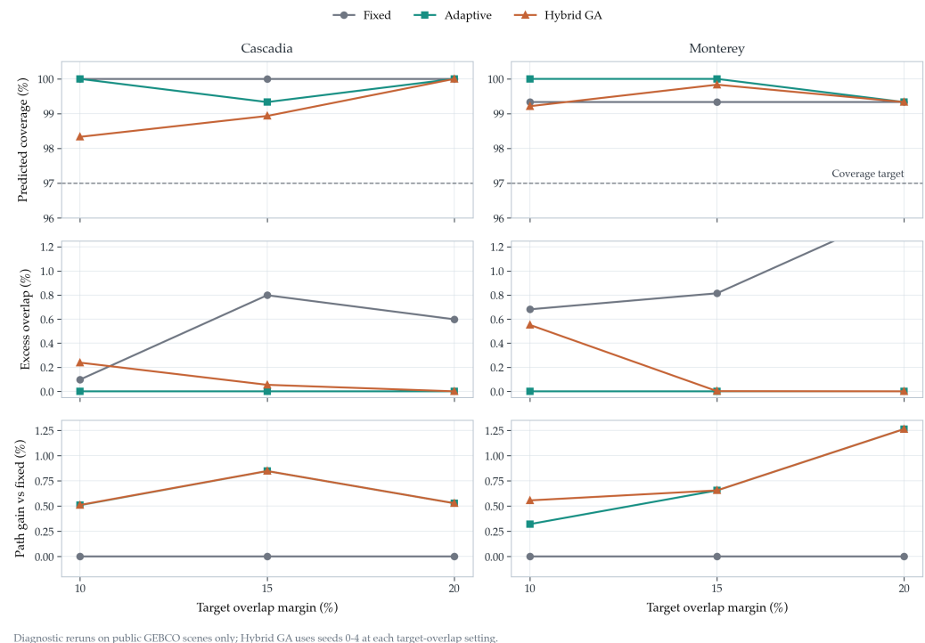
Figure 9. Public-scene target-overlap sensitivity diagnostic. Fixed-Spacing, Adaptive Spacing without GA, and Full Geometry-Aware Hybrid GA are rerun on the two GEBCO public scenes at target-overlap margins of 10, 15, and 20 percent using the same reported evaluator and a 120° MBES opening angle. Hybrid GA reports the mean over seeds 0–4 for this diagnostic; the main benchmark results remain the 20-seed values reported in this study. The figure shows that all tested public layouts remain feasible, but the selected line family and path gain depend on the declared design margin.
