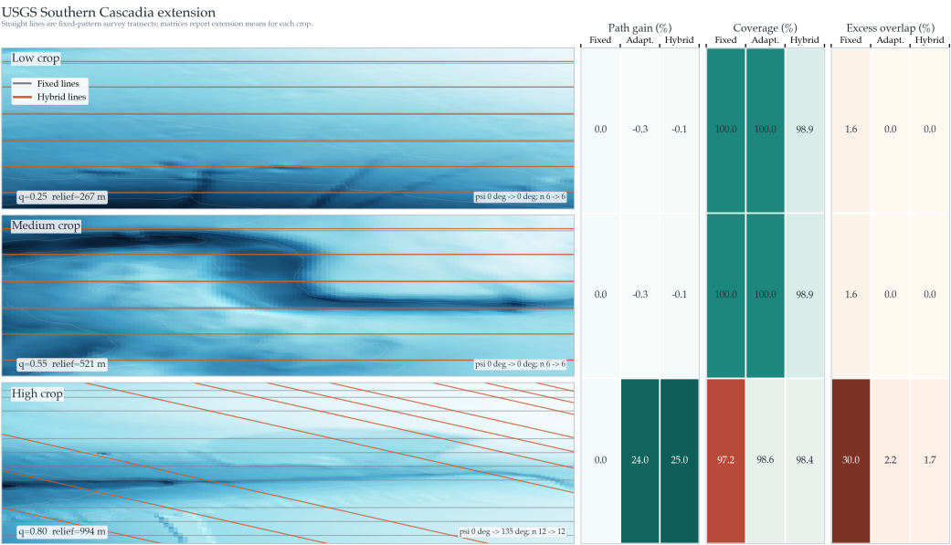
Figure 12. Independent USGS Southern Cascadia 30 m multibeam-derived public-grid extension. The left column shows the three selected crops with Fixed-Spacing and representative Hybrid GA line families, ordered by empirical terrain complexity from low to high. These plotted straight transects are the planned fixed-pattern survey-line families, not free-form vehicle trajectories. The three right-side matrices report benchmark means for path gain relative to Fixed-Spacing, predicted coverage, and excess-overlap violation recomputed from the extension CSV/JSON outputs. A wider map column preserves terrain readability while the matrices retain the scene-by-method comparison. The extension remains a public-grid numerical check, not an additional sea-trial or mission-log validation.
