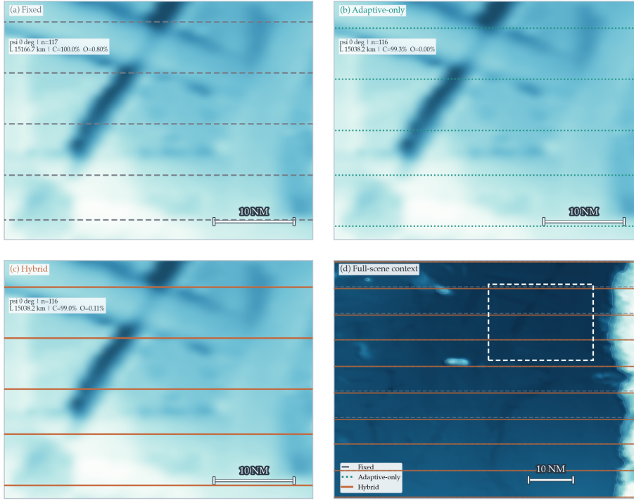
Figure 3. GEBCO Cascadia Margin public-scene comparison on the benchmark reported in this study. Panels (a)–(c) show Fixed-Spacing, Adaptive Spacing without GA, and Full Geometry-Aware Hybrid GA on a shared relief-focused zoom window, so the line-placement differences can be read without the large empty basin region dominating the figure. Panel (d) restores the full-scene context and marks the zoom window location. Panel (e) reports the heading, line count, path length L , predicted coverage C , and excess-overlap violation O computed from the full scene, while panel (f) converts those values into relative path gain and remaining overlap against Fixed-Spacing. Only representative lines are drawn for readability, but all reported metrics use the full layouts. All three methods retain the 0^\circ sweep family in this control scene.
