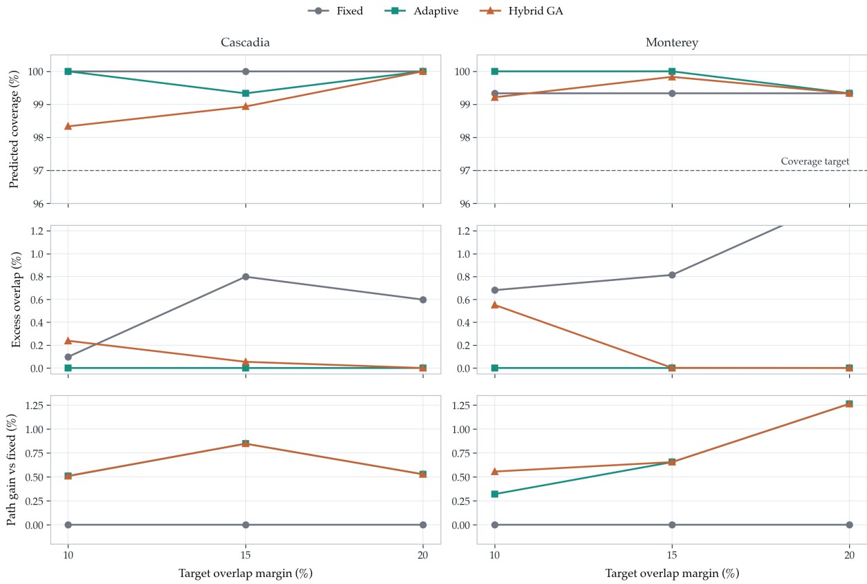
Figure 9. Public-scene target-overlap sensitivity diagnostic. Fixed-Spacing, Adaptive Spacing without GA, and Full Geometry-Aware Hybrid GA are rerun on the two GEBCO public scenes at target-overlap margins of 10, 15, and 20 percent using the same reported evaluator and a 120° MBES opening angle. Hybrid GA reports the mean over seeds 0–4 for this diagnostic; the main benchmark results remain the 20-seed values reported in this study. The figure shows that all tested public layouts remain feasible, but the selected line family and path gain depend on the declared design margin.
