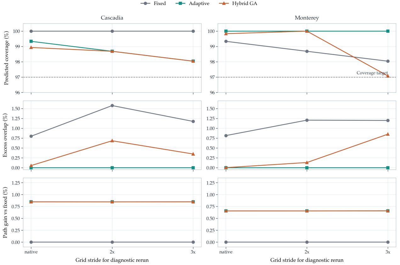
Figure 10. Public-scene grid-resolution sensitivity diagnostic. The same three public-scene methods are rerun on the native GEBCO-derived grids and on 2\times and 3\times strided downsampled grids using the reported evaluator. Hybrid GA reports seeds 0–4 for this diagnostic, whereas the main benchmark remains the native-grid 20-seed benchmark used in this study. The Monterey 3\times case exposes a resolution-dependent coverage boundary for the Hybrid GA, so the diagnostic should be interpreted as a planning-evaluator sensitivity check rather than as field-performance evidence.
