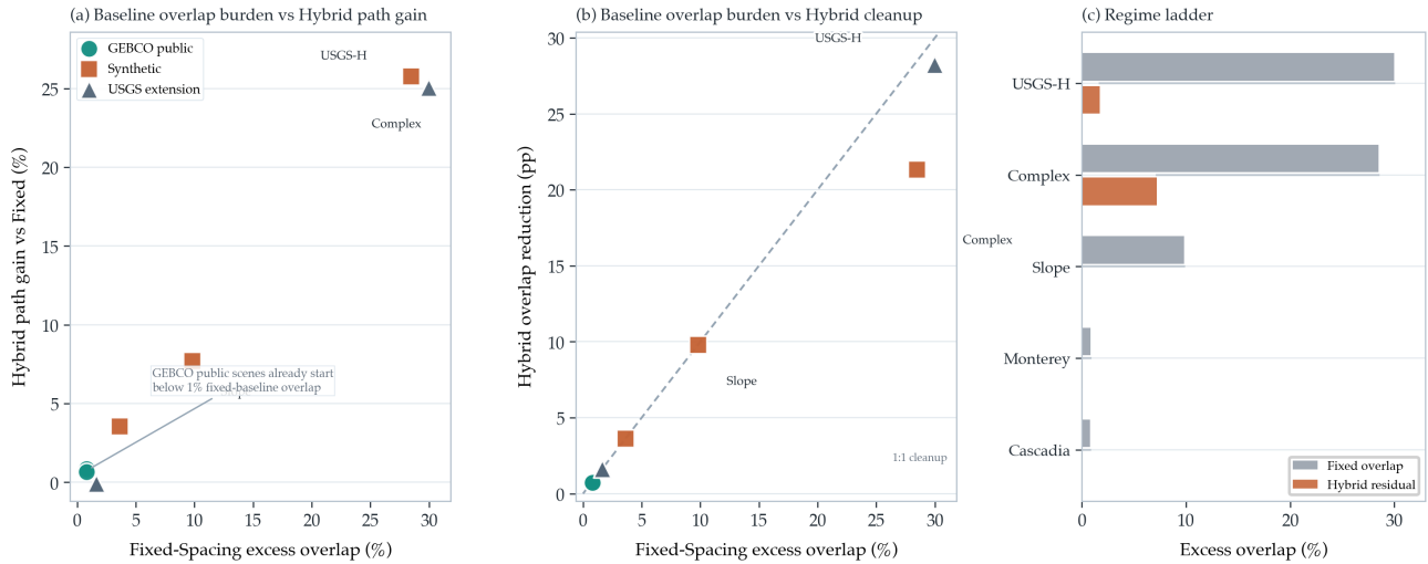
Figure 6. Scene-level regime diagnostic linking the Fixed-Spacing baseline to the observed Hybrid benefit. Each point is one scene from either the reported main benchmark or the separate USGS 30 m extension. Panel (a) plots Fixed-Spacing excess-overlap burden against Hybrid path gain relative to Fixed-Spacing. Panel (b) plots the same burden against Hybrid overlap reduction. Panel (c) gives a ranked overlap-regime ladder, comparing the Fixed-Spacing burden with the Hybrid residual on representative scenes. The GEBCO public scenes cluster in a low-overlap regime below 1 percent excess overlap, whereas Complex Terrain and the high-complexity USGS crop start near 30 percent excess overlap and therefore show the largest geometry-aware gains. The USGS points strengthen the mechanism interpretation but are not merged into the main benchmark averages reported elsewhere in the paper.
