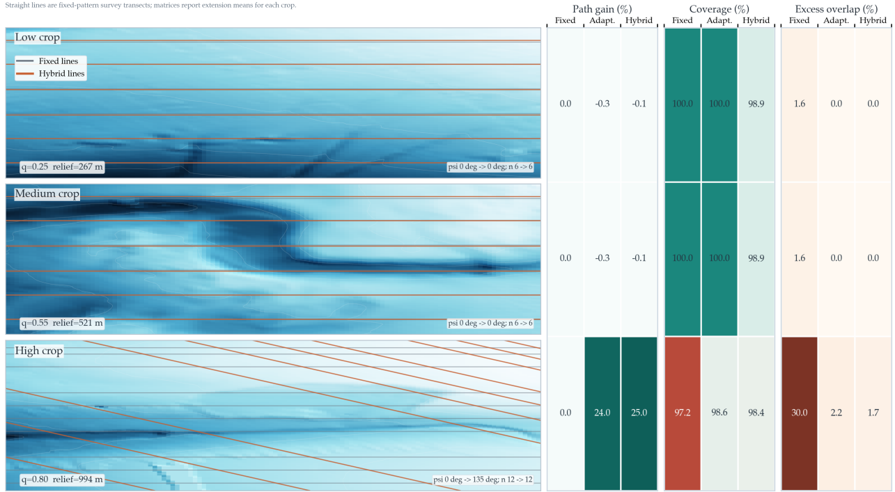
Figure 12. Independent USGS Southern Cascadia 30 m multibeam-derived public-grid extension. The left column shows the three selected crops with Fixed-Spacing and representative Hybrid GA line families, ordered by empirical terrain complexity from low to high. These plotted straight transects are the planned fixed-pattern survey-line families, not free-form vehicle trajectories. The three right-side matrices report benchmark means for path gain relative to Fixed-Spacing, predicted coverage, and excess-overlap violation recomputed from the extension CSV/JSON outputs. A wider map column preserves terrain readability while the matrices retain the scene-by-method comparison. The extension remains a public-grid numerical check, not an additional sea-trial or mission-log validation.
