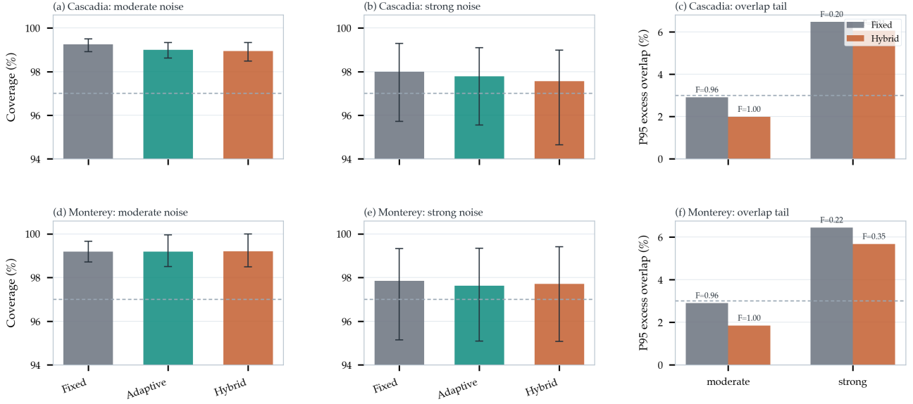
Figure 11. Execution-uncertainty replay on the two public GEBCO layouts. Panels (a), (b), (d), and (e) show mean predicted coverage with 5–95 percent Monte Carlo intervals under moderate and strong post-planning perturbations. Panels (c) and (f) show the 95th-percentile excess-overlap tail and the feasibility rate F for Fixed-Spacing and Hybrid GA. Under moderate perturbations, Hybrid GA remains feasible in 299/300 Cascadia trials and 300/300 Monterey trials; under strong perturbations, all methods lose substantial feasibility margin, indicating that execution-aware safety margins would be needed before field use.
