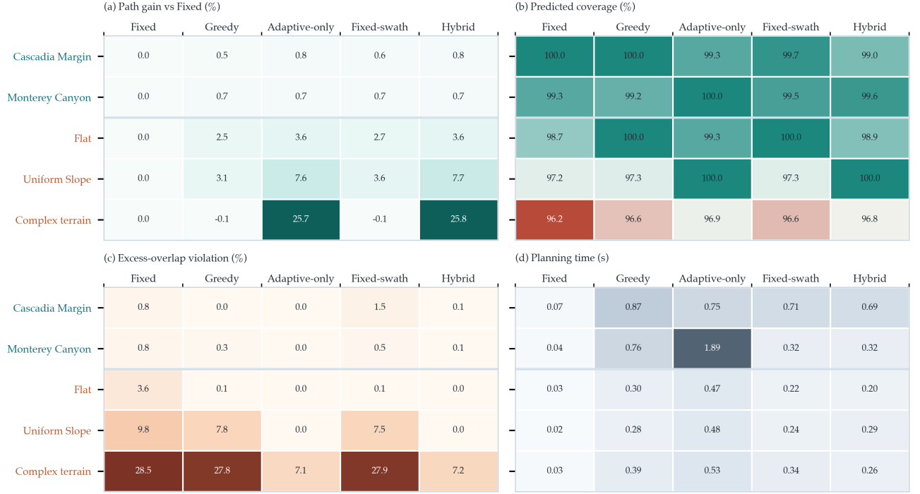
Figure 5. Cross-scene metric matrix from the reported benchmark. Each panel is a scene-by-method heatmap of benchmark means: path gain relative to Fixed-Spacing, predicted coverage, excess-overlap violation, and planning time. The top two rows are the public GEBCO scenes and the bottom three rows are synthetic stress tests, so the figure exposes both the public-data pattern and the complex-terrain failure boundary in one compact view. Stochastic GA methods report 20-seed means, and all coverage values are numerical predictions rather than field measurements.
