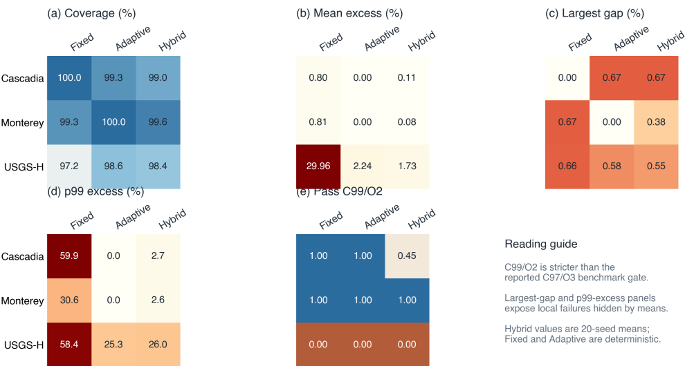
Figure 15. Threshold and local-failure diagnostic for the two primary GEBCO scenes and the USGS high-complexity crop. The figure reports mean coverage, mean excess-overlap violation, largest connected uncovered patch, the 99th-percentile cellwise excess-overlap tail, and the pass rate under a stricter C99/O2 screen requiring at least 99 percent predicted coverage and at most 2 percent mean excess overlap. Hybrid GA values are 20-seed means; Fixed-Spacing and Adaptive Spacing without GA are deterministic. The diagnostic is a raster-evaluator audit designed to expose local failures hidden by scene-level means; it is not hydrographic QA or a field-survey acceptance test.
