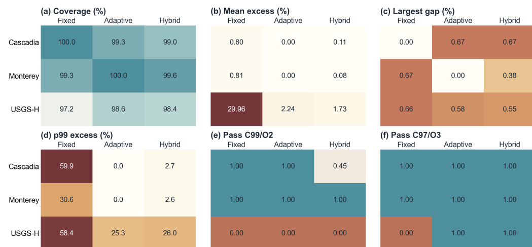
Figure 15. Threshold and local-failure diagnostic for the two primary GEBCO scenes and the USGS high-complexity crop. The figure reports mean coverage, mean excess-overlap violation, largest connected uncovered patch, the 99th-percentile cellwise excess-overlap tail, and pass rates under both the stricter C99/O2 screen and the manuscript’s default C97/O3 benchmark gate. Hybrid GA values are 20-seed means; Fixed-Spacing and Adaptive Spacing without GA are deterministic. The diagnostic is a raster-evaluator audit designed to expose local failures hidden by scene-level means; it is not hydrographic QA or a field-survey acceptance test.
