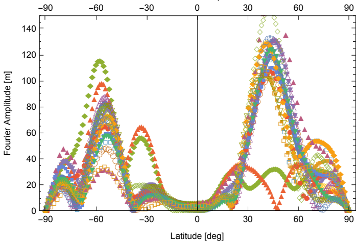
500hPa Wave 1 Amplitude JAN
