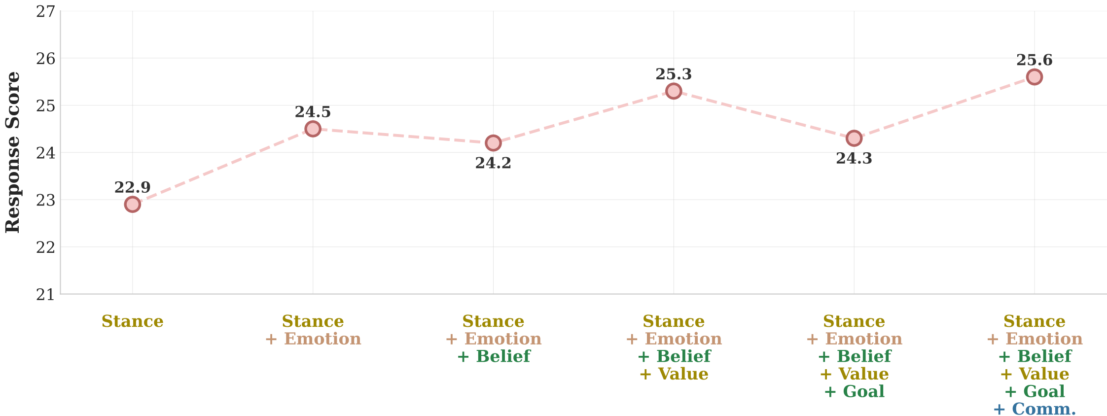
Response Score Saturates as More State Dimensions Are Added on HUMANUAL-Opinion
