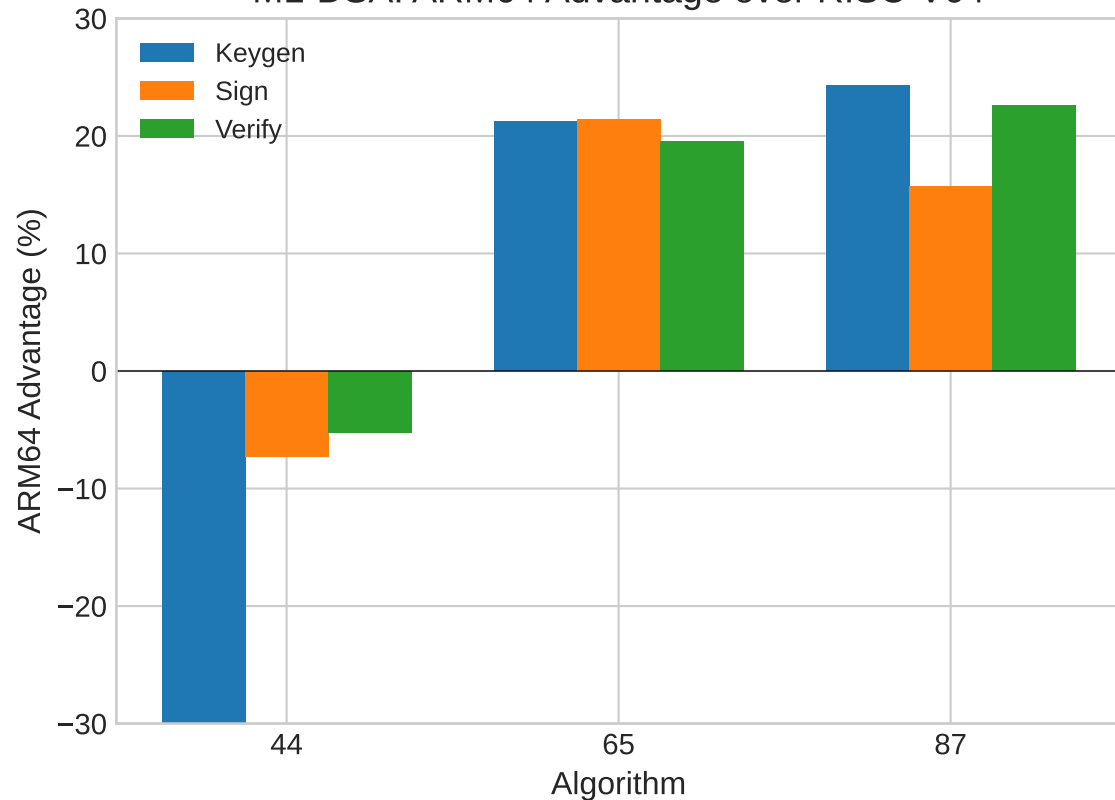
ML-DSA: ARM64 Advantage over RISC-V64
