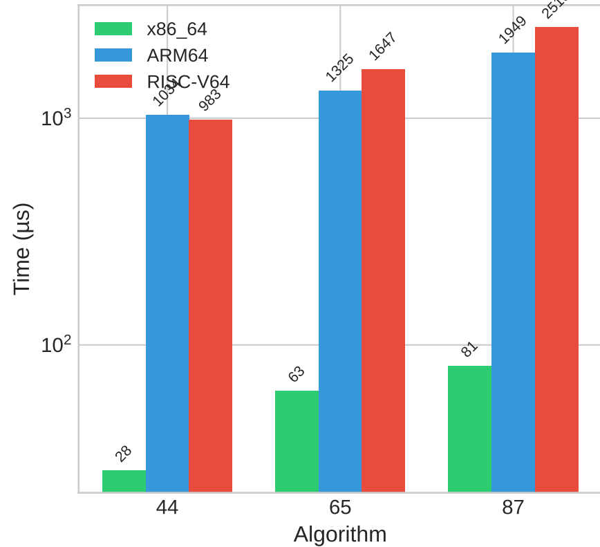
ML-DSA Verify
