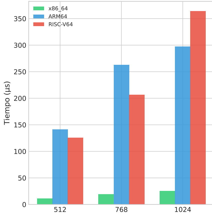
ML-DSA Keygen
