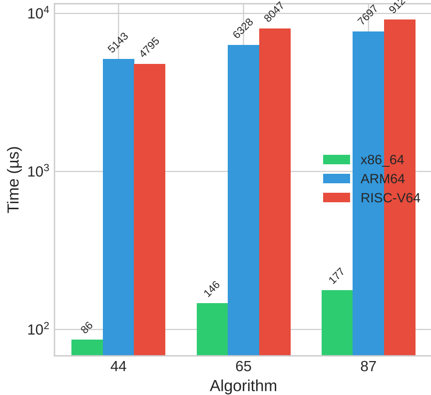
ML-DSA Sign
