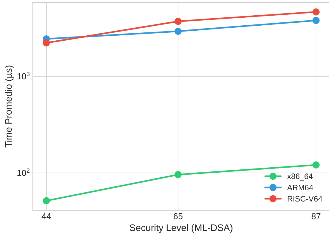
ML-DSA: Scaling by Level
