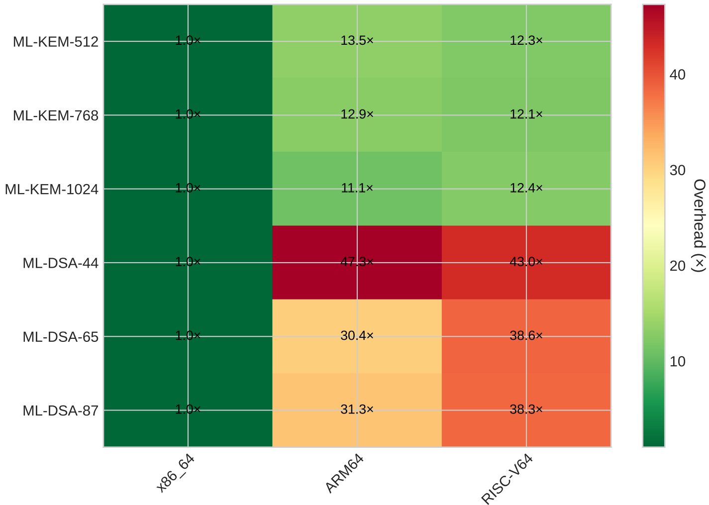
Overhead Relative vs Native x86_64 (1.0x = equal performance)
