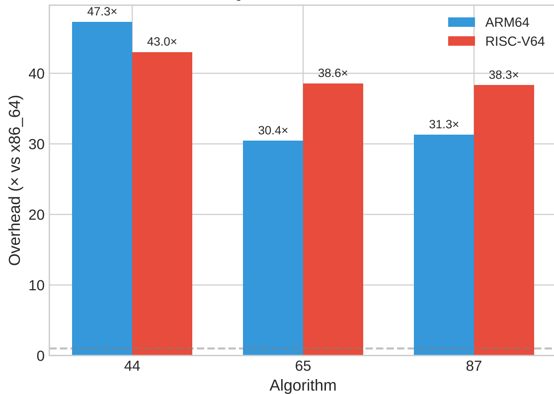
ML-DSA: QEMU Emulation Overhead
