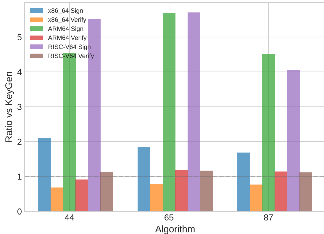
ML-DSA: Relative Operation Cost
