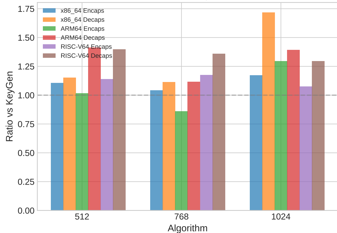
ML-KEM: Relative Operation Cost
