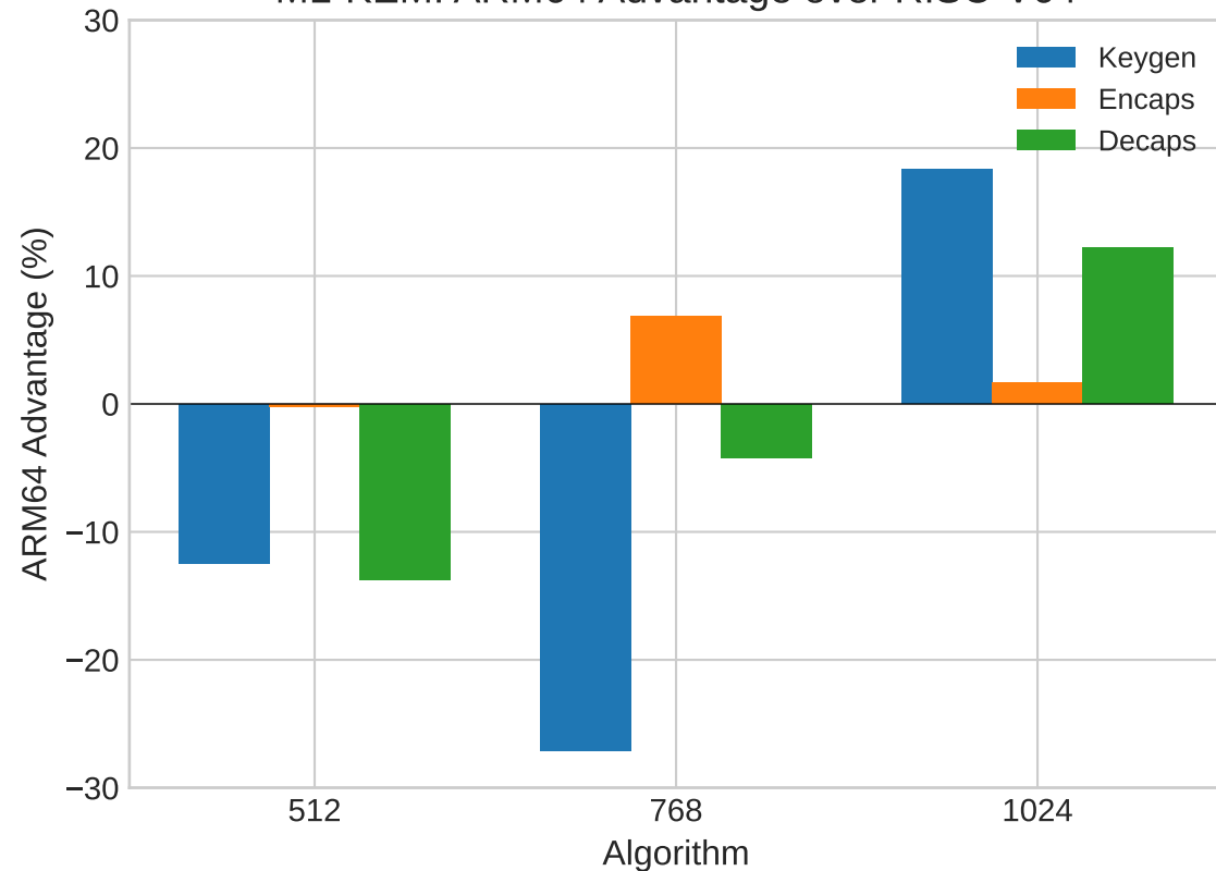
ML-KEM: ARM64 Advantage over RISC-V64
