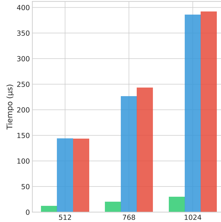
ML-DSA Sign
