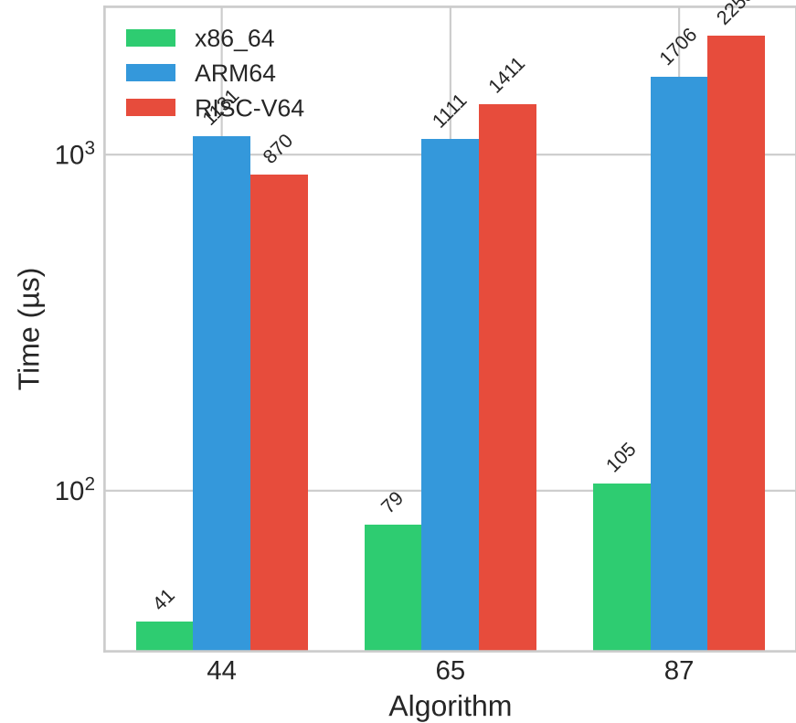
ML-DSA KeyGen
