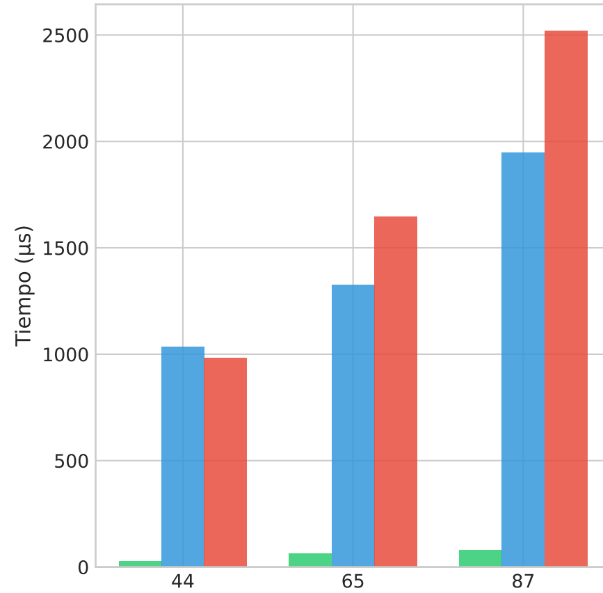
ML-DSA Verify
