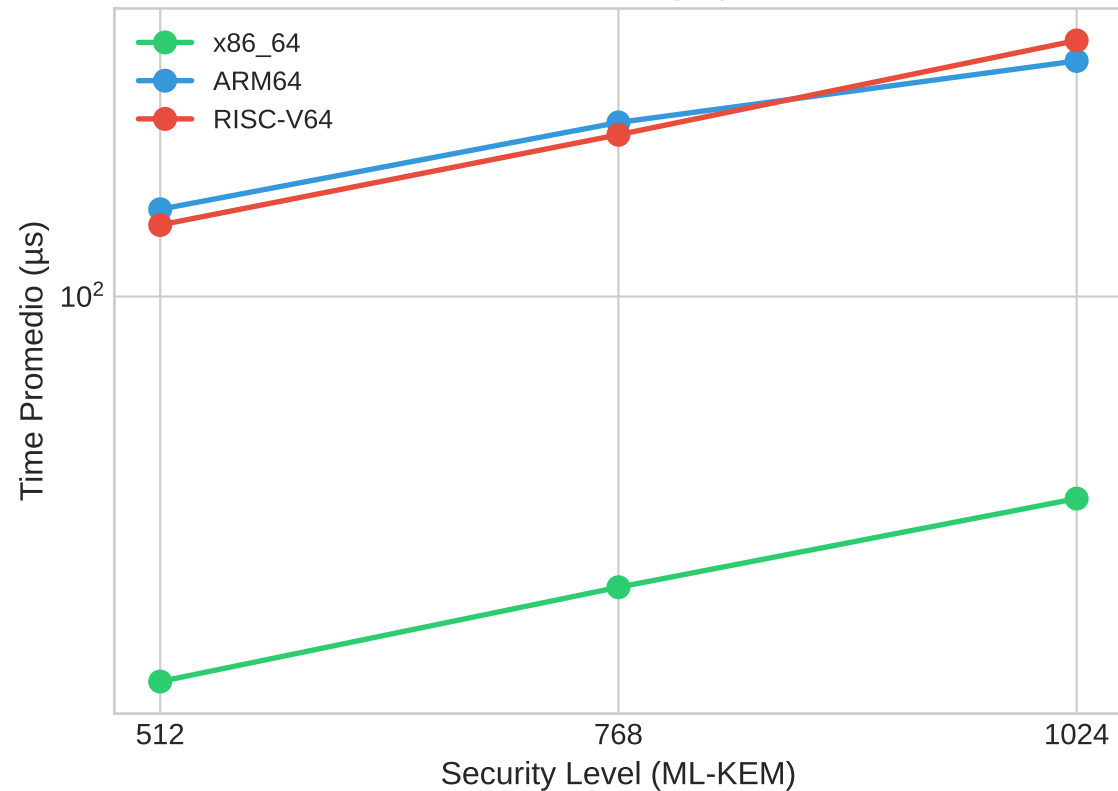
ML-KEM: Scaling by Level
