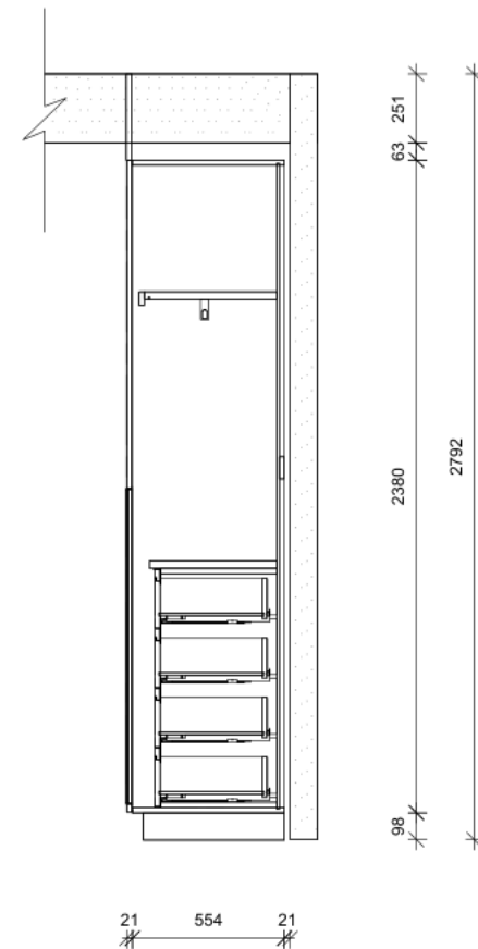
SECTION 1
