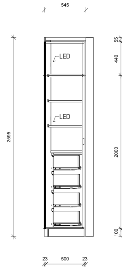
SECTION 2
