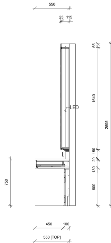
SECTION 3
