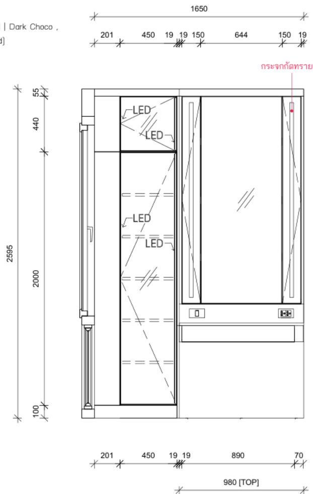
ELEVATION C
