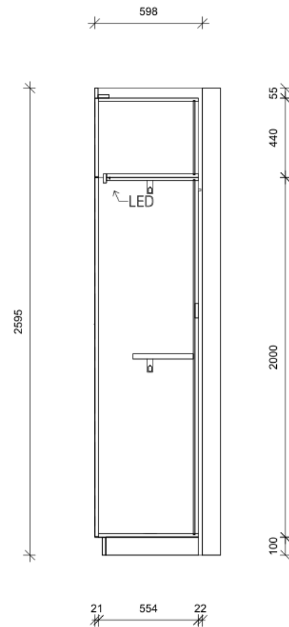
SECTION 1
