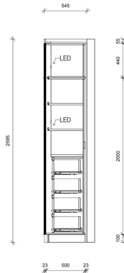
SECTION 2
