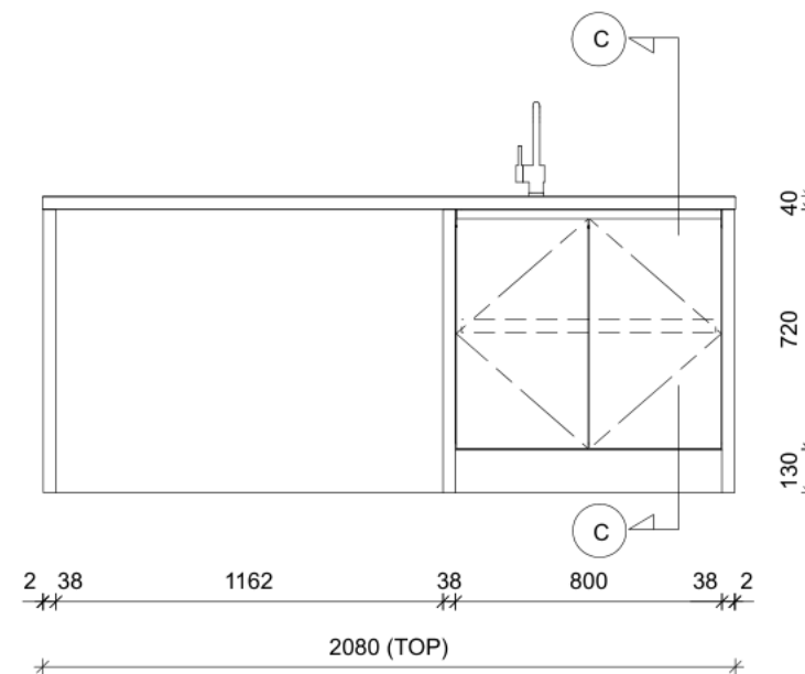
ELEVATION C
