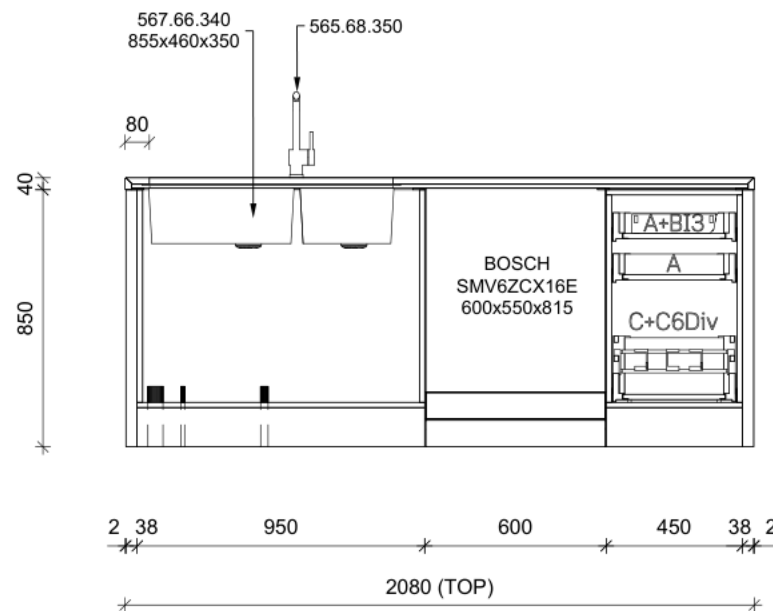
SECTION B
