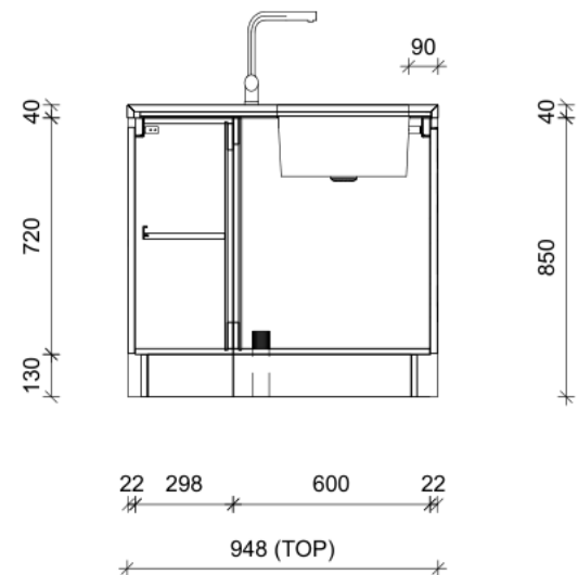
SECTION C
