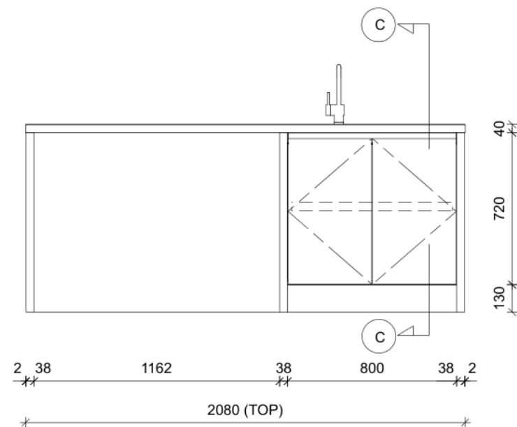
ELEVATION C
