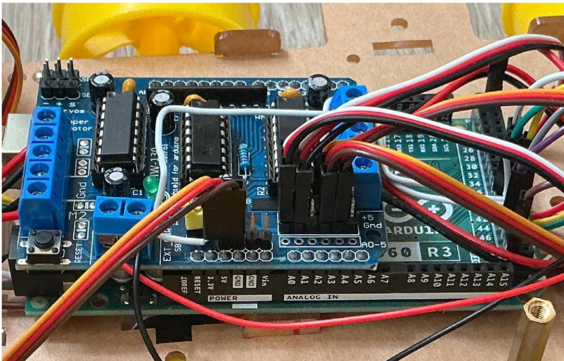
Figure B-8: Soldering and wiring on Alex's Motor shield & Arduino
