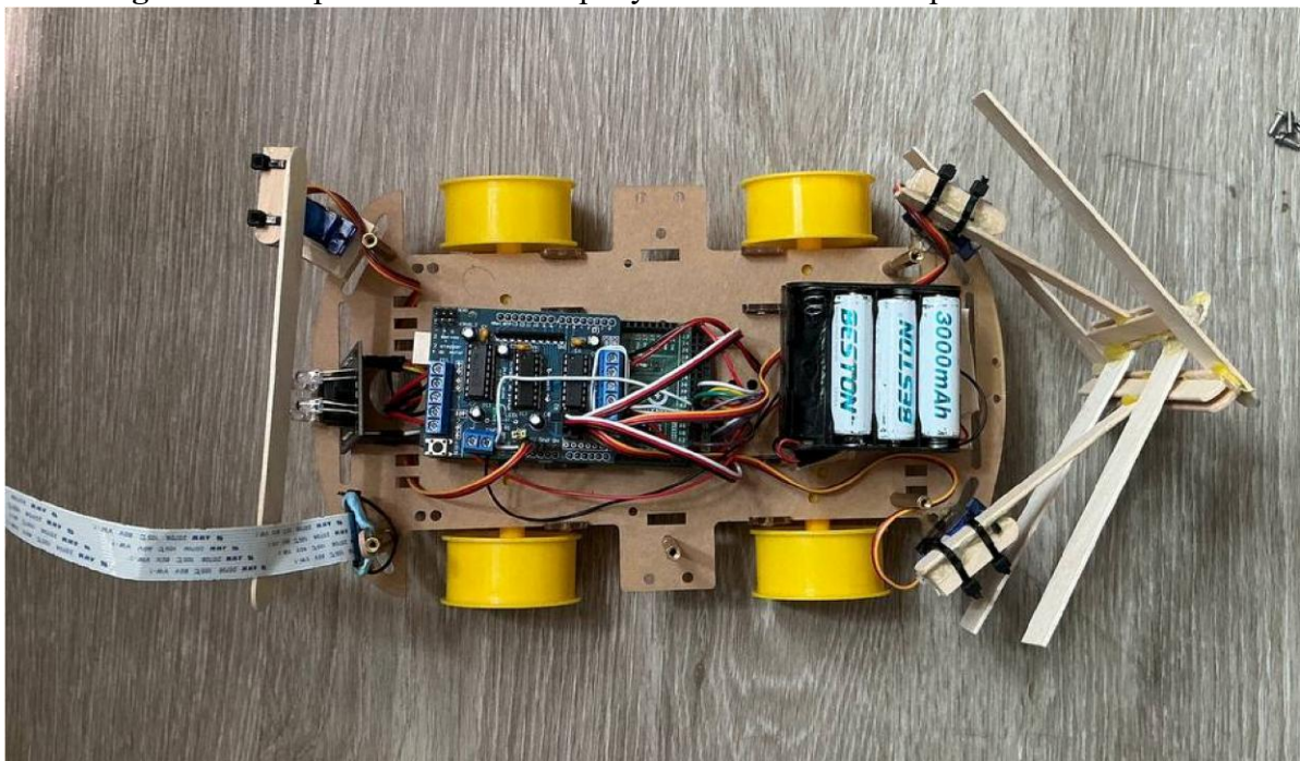
Figure B-6: Top view of Alex's base layer with closed dispenser and Claws
