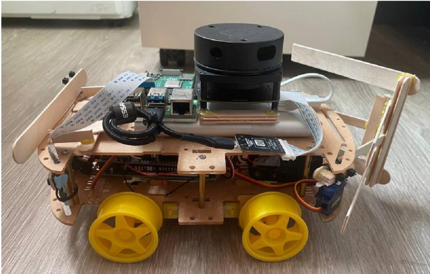
Figure B-1: Alex's Right Side
