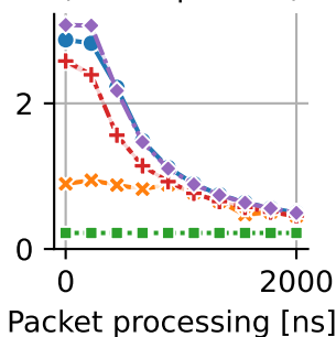
(b) Throughput (1500B packets)
