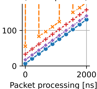
(e) Latency (1500B packets)
