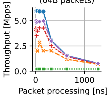
(a) Throughput (64B packets)
