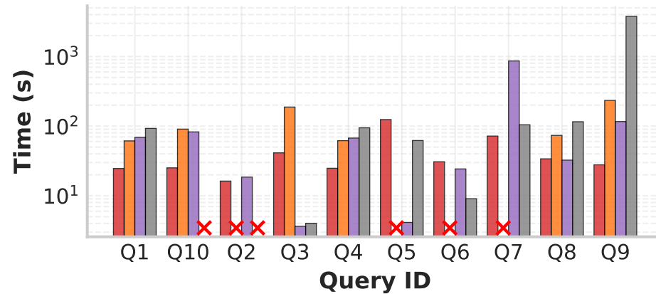
Latency
