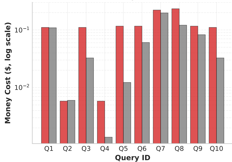
Money Cost
