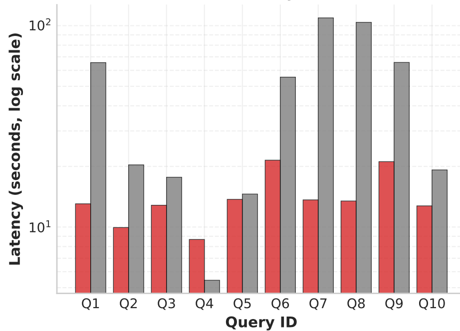
Latency
