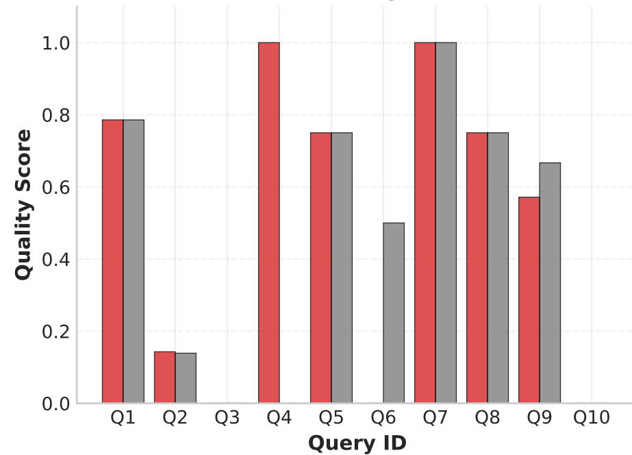
Quality
