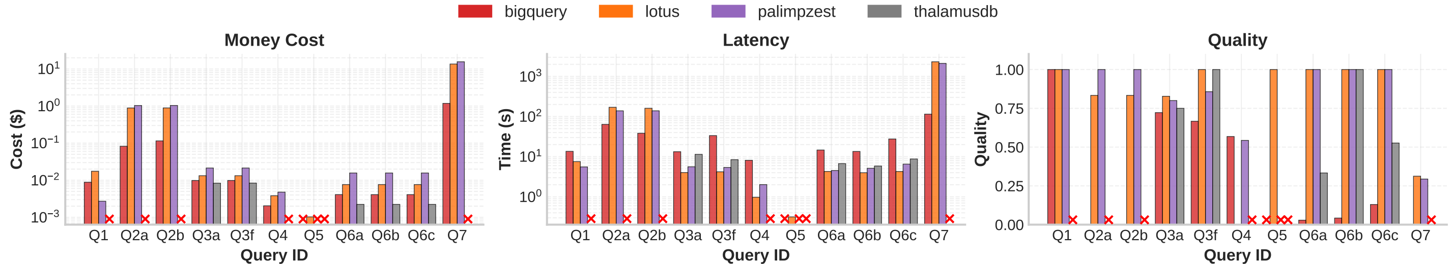
(e) MMQA Scenario
