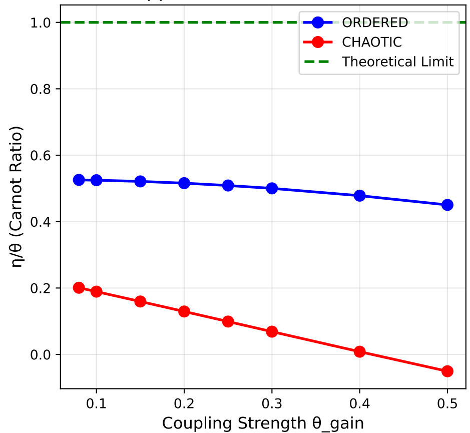
Approach to Universal Limit
