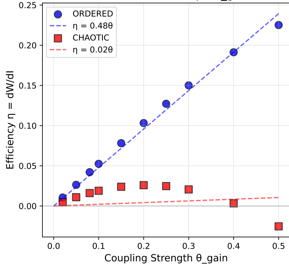
The Carnot Bound: \eta \propto \theta_{\text{gain}}
