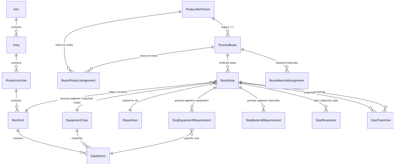
MES Routing &amp; ISA-95 Physical Model ER Diagram
