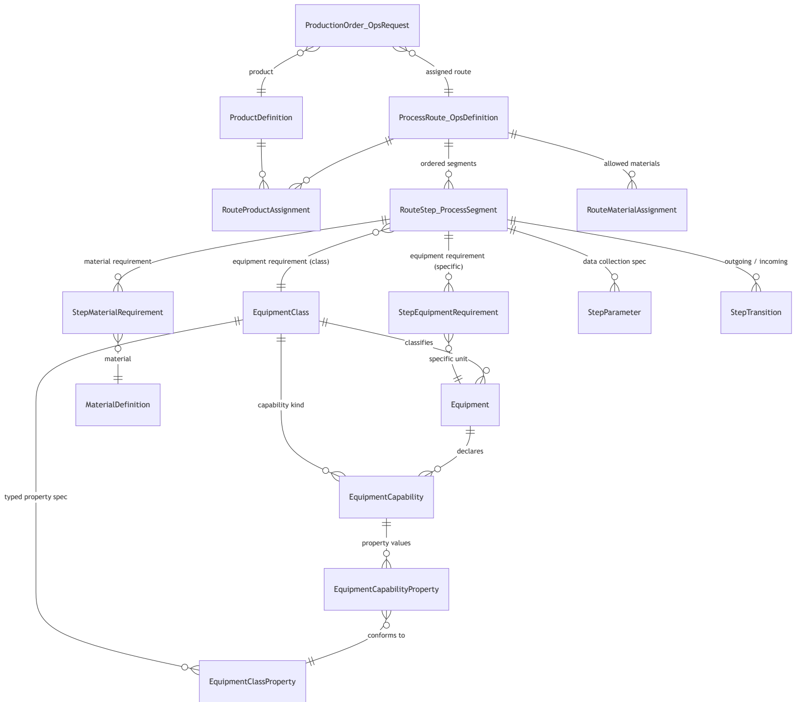
ISA-95 Part 2 ER Diagram (as implemented in MES AI)
