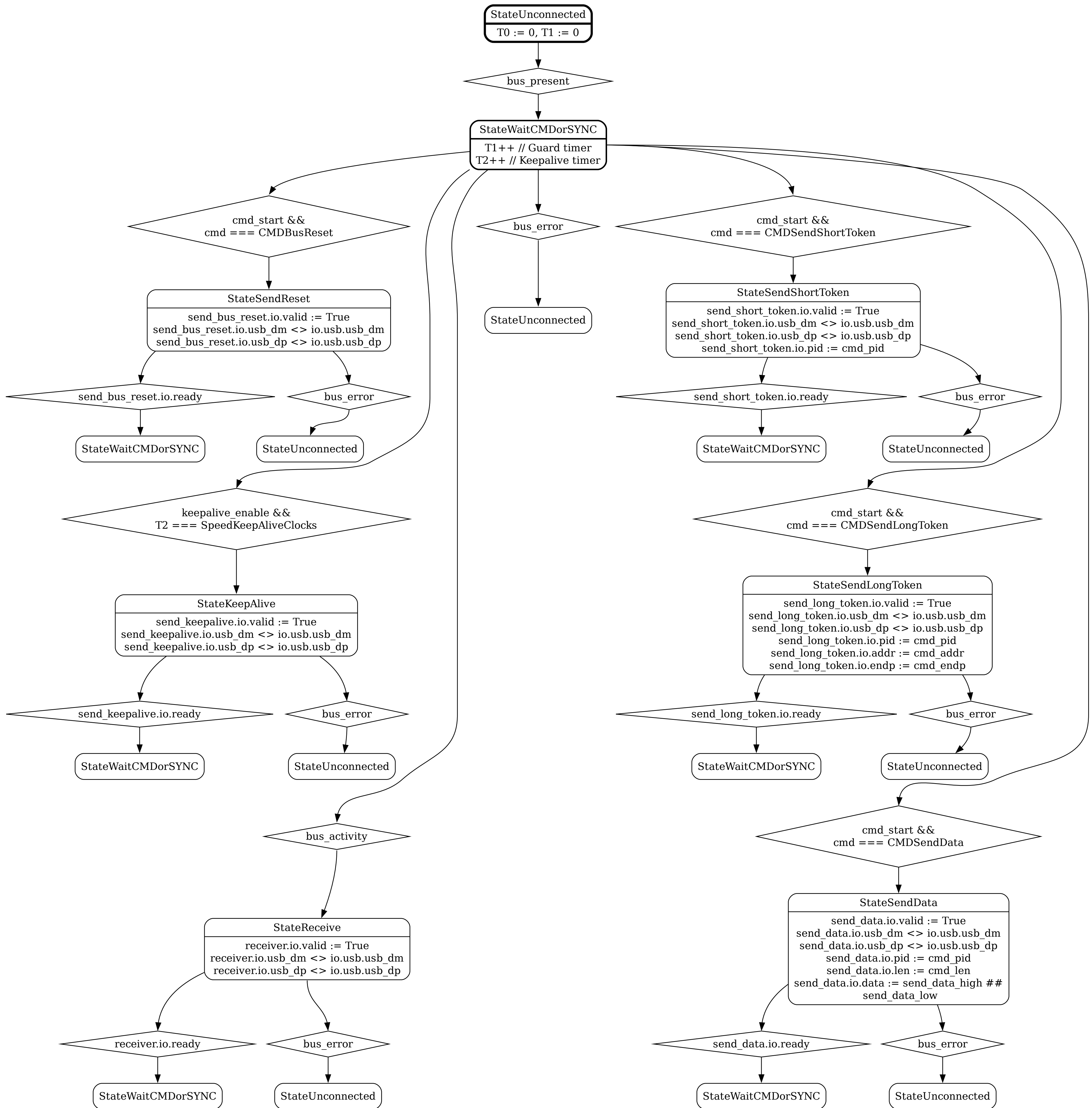
USB 1.0 Controller Main FSM
