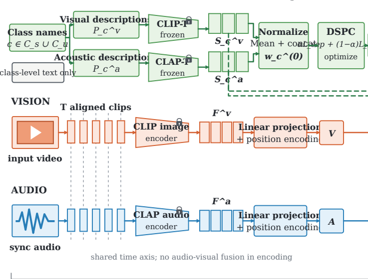
(a) Semantic and Feature Encoding
