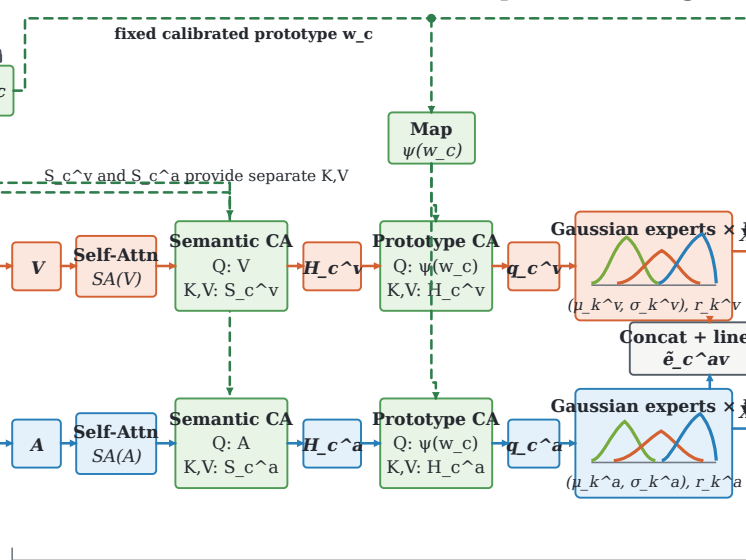
(b) Semantic-Guided Gaussian Temporal Grounding
