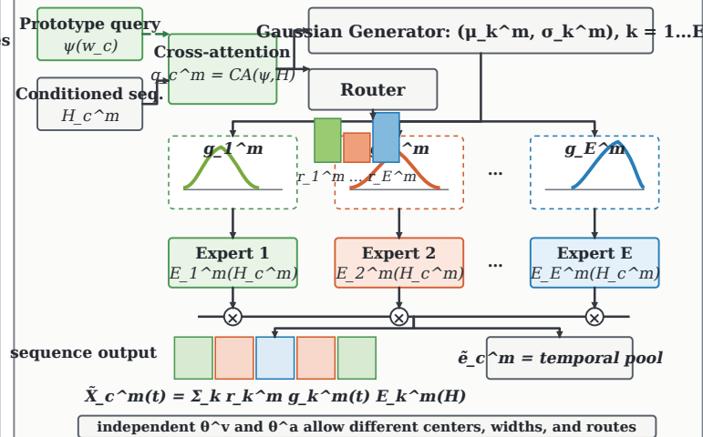
② SGTG · Semantic-Guided Gaussian Temporal Grounding
