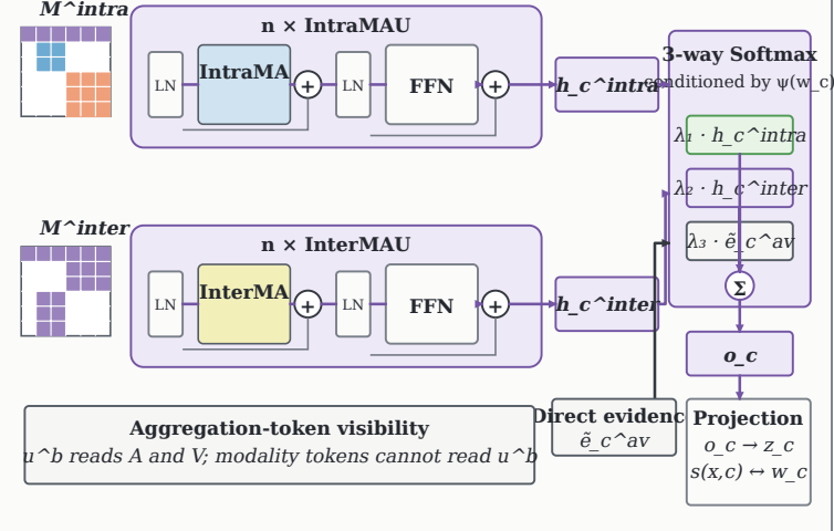
③ DMIF · Decoupled Modality Interaction and Gated Fusion
