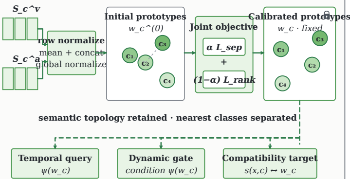
① DSPC · Discriminative Semantic Prototype Calibration
