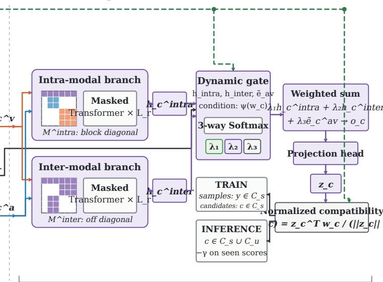
(c) Decoupled Interaction, Fusion and Prediction
