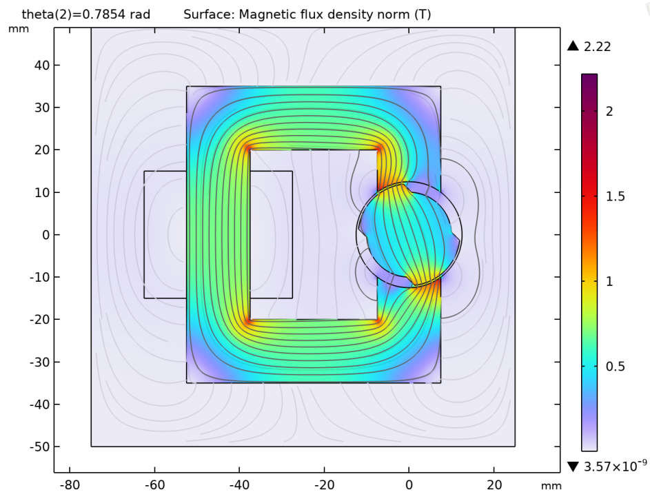
Figure 15: Flux density vector plot for the nonlinear material model, \theta = 45^\circ .
