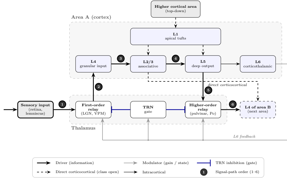
Figure 1.1: The cortico-thalamo-cortical loop and the canonical cortical column, traced as a numbered flow. (1) Sensory input reaches a first-order relay, which (2) drives layer 4. (3–4) The column processes it through the canonical intracolumnar flow (L4 \rightarrow L2/3 \rightarrow L5); layer 5 also projects to layer 6 (thin, intracortical). (5–6) Layer 5 sends a driving projection to a higher-order relay, which drives layer 4 of the next cortical area (the transthalamic route). In parallel, layer 6 returns a modulatory projection (thin grey) to both relays and the TRN, and the TRN gates both relays (blue, bar-ended). Direct corticocortical projections (dashed, class open) run alongside the transthalamic route: feedforward from L2/3 to layer 4 of the next area, and top-down feedback from a higher cortical area onto the apical tufts of L2/3 and L5 pyramidal cells in layer 1. The relays’ collateral input to the TRN is omitted for clarity. Connection classes follow Sherman and Guillery [sherman1998drivers, sherman2013functional].
