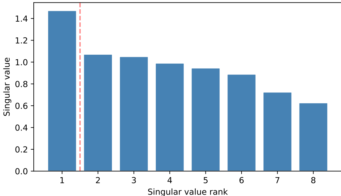
Displacement matrix A — singular value spectrum \rho = \lambda_1/\lambda_2 = 1.37
