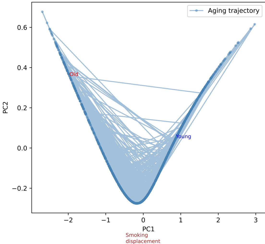
Smoking vs aging trajectory \cos \text{ similarity} = +0.176 , \text{angle} = 79.9^\circ
