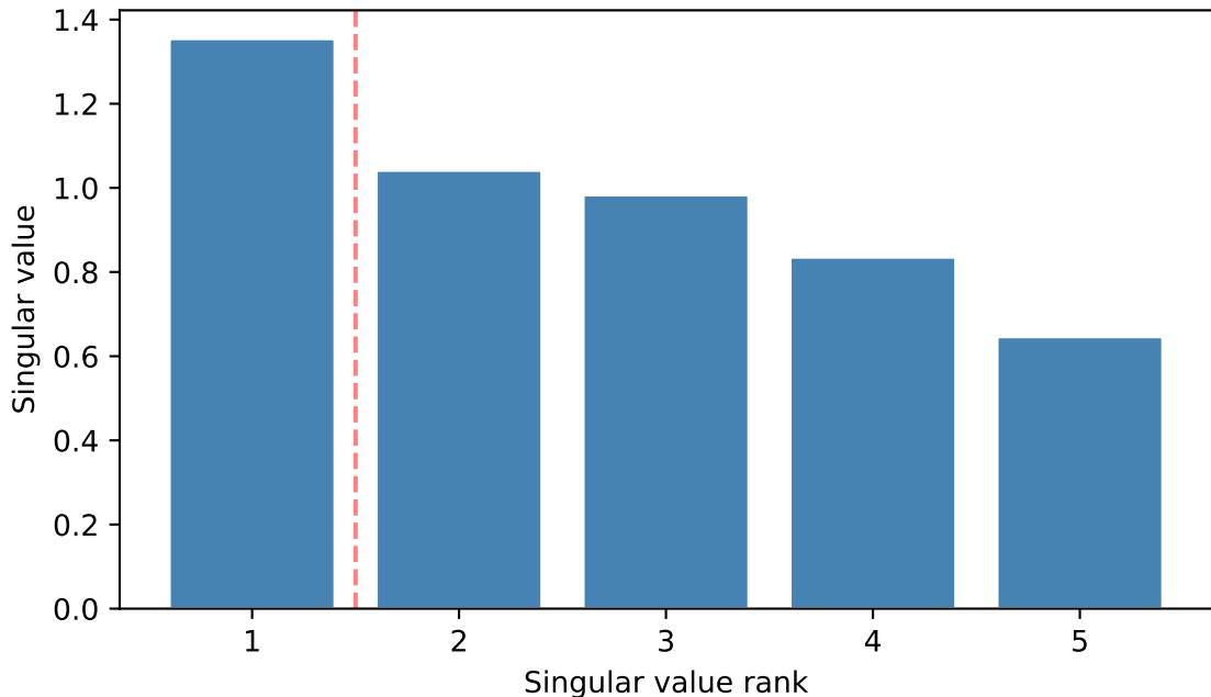
Displacement matrix A — singular value spectrum \rho = \lambda_1/\lambda_2 = 1.30
