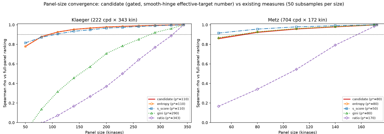
Figure 7: Panel-size convergence of the candidate measure compared with the four existing definitions, on the two sparse-coverage datasets (Klaeger, left; Metz, right; 50 random subpanels per size). Curves show the mean Spearman correlation between the ranking computed on a random subpanel and the full-panel ranking; p^* (legend) is the smallest panel reaching mean \rho > 0.90 .
