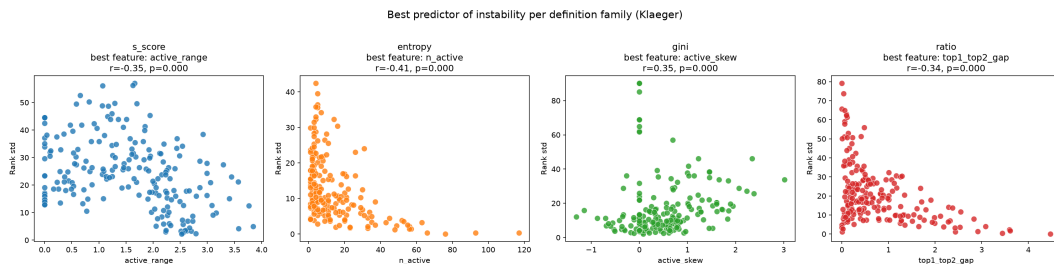
Figure 3: Best predictor of rank instability within each definition family (Klaeger dataset, active compounds, n = 206 ). Ratio instability is best predicted by the top 1 –top 2 affinity gap; entropy, Gini, and S-score instability are best predicted by features of the active affinity distribution.
