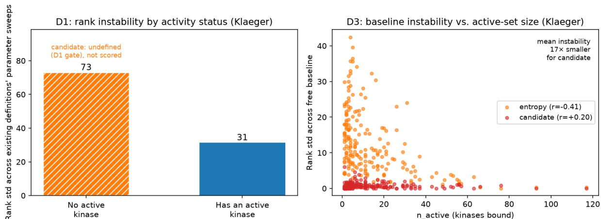
Figure 6: The two failure modes the candidate measure repairs (Klaeger). Left (D1) : rank instability (std across the existing definitions’ parameter sweeps) for compounds with no binding above the activity threshold versus compounds with at least one active kinase. Right (D3) : per-compound rank instability under the free activity baseline, against the number of active kinases, for the entropy and for the candidate.
