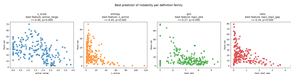
Figure 3. Best predictor of rank instability within each definition family (Klaeger dataset, active compounds, n = 206 ). Ratio instability is best predicted by the top_1 – top_2 affinity gap; entropy, Gini, and S-score instability are best predicted by features of the active affinity distribution.
