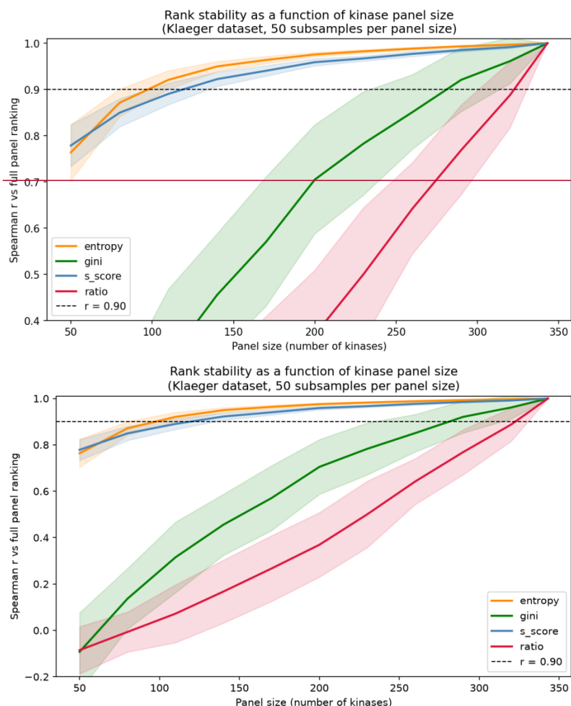
Figure 35. Mean Spearman correlation between rankings computed on random kinase subpanels and rankings on the full Klaeger panel (343 kinases), as a function of subpanel size. Shaded bands indicate \pm 1 standard deviation across 50 subsamples. The dashed line marks r = 0.90 . Entropy and S-score rankings stabilize at approximately 110–140 kinases; Gini requires approximately 290 kinases; ratio does not reach r = 0.90 at any practically used panel size.
