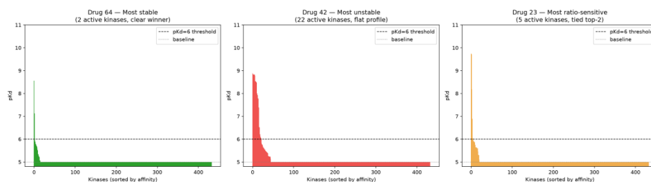
Figure 4. Representative binding profiles illustrating the three instability types. Left: Drug 64 (Davis), most stable ( \sigma = 1.6 ), two active kinases. Center: Drug 42 (Davis), most unstable ( \sigma = 19.3 ), 22 active kinases at near-identical affinities. Right: Drug 23 (Davis), most ratio-sensitive, five active kinases including two near-tied top targets ( \Delta \text{p}K_d = 0.023 ). Dashed line: \text{p}K_d = 6 activity threshold; dotted line: \text{p}K_d = 5 assay floor.
