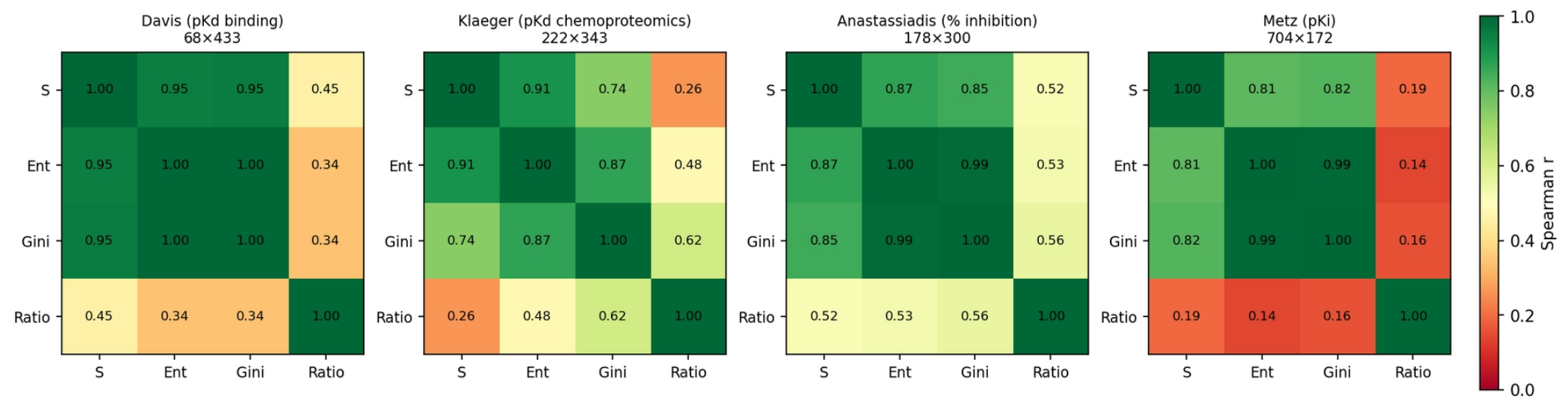
Two-family structure across four datasets: S-score/entropy/Gini cluster; ratio is the consistent outlier
