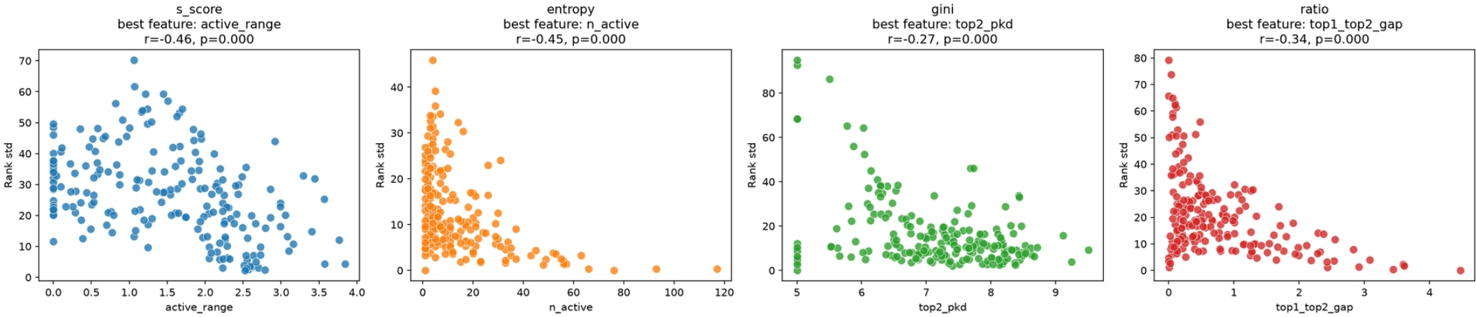
Best predictor of instability per definition family
