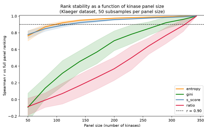
Figure 5. Mean Spearman correlation between rankings computed on random kinase subpanels and rankings on the full Klaeger panel (343 kinases), as a function of subpanel size. Shaded bands indicate \pm 1 standard deviation across 50 subsamples. The dashed line marks r = 0.90 . Entropy and S-score rankings stabilize at approximately 110–140 kinases; Gini requires approximately 290 kinases; ratio does not reach r = 0.90 at any practically used panel size.
