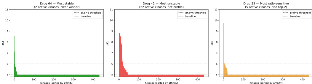
Figure 4: Representative binding profiles illustrating the three instability types. Left: Drug 64 (Davis), most stable ( \sigma = 1.6 ), two active kinases. Center: Drug 42 (Davis), most unstable ( \sigma = 19.3 ), 22 active kinases at near-identical affinities. Right: Drug 23 (Davis), most ratio-sensitive, five active kinases including two near-tied top targets ( \Delta pK_d = 0.023 ). Dashed line: pK_d = 6 activity threshold; dotted line: pK_d = 5 assay floor.
