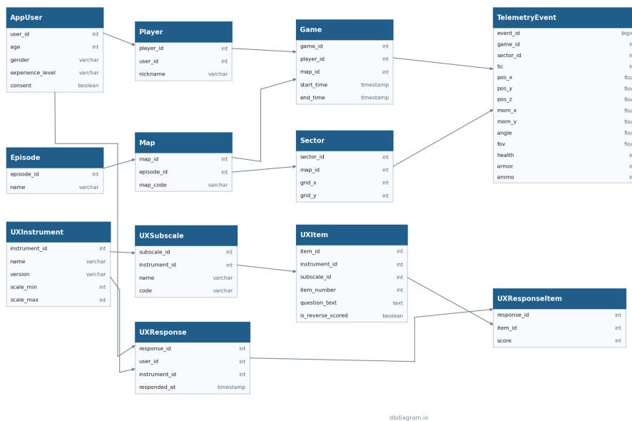
Figure 1: Entity-Relation Diagram *
