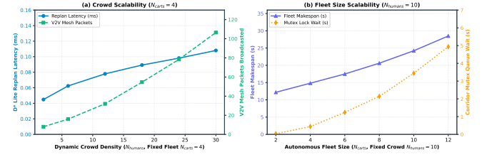
Fig. 10: Decoupled fleet scalability evaluations: (a) Incremental D* Lite replanning latency and V2V mesh broadcast packets vs. dynamic crowd density ( N_{\text{humans}} \in [2..30] , fixed fleet N = 4 ); (b) Fleet makespan and single-file corridor mutex queueing wait time vs. autonomous fleet size ( N_{\text{carts}} \in [2..12] , fixed crowd N = 10 ).
