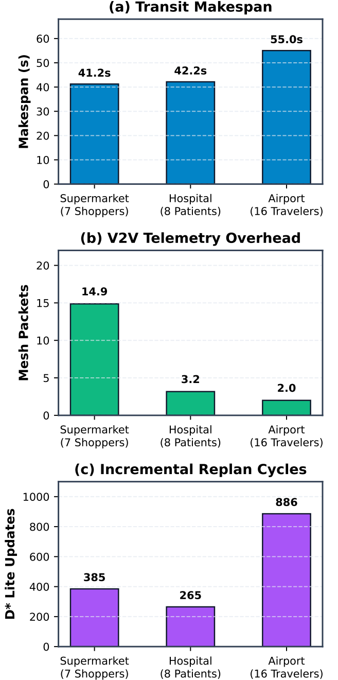
Fig. 9: Multi-domain fleet performance across Supermarket, Hospital, and Airport environments on (a) Makespan, (b) V2V Mesh Packets, and (c) Incremental Replan Cycles.
