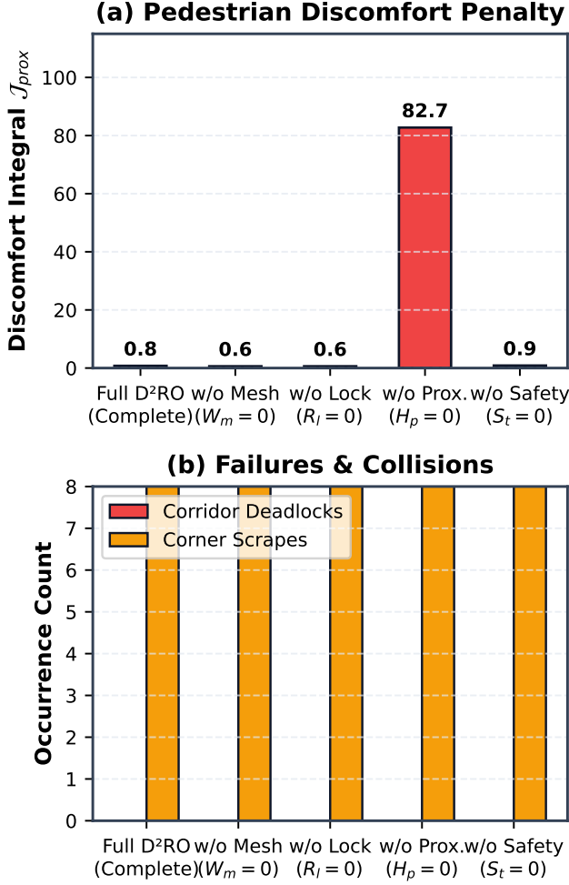
Fig. 8: Component ablation study evaluating (a) Discomfort Integral and (b) Corridor Deadlocks & Shelf Corner Scrapes across the 5 cost configurations.
