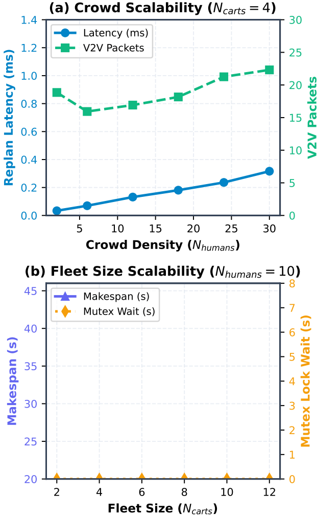
Fig. 10: Decoupled fleet scalability evaluations: (a) Incremental D* Lite replanning latency and V2V mesh broadcast packets vs. dynamic crowd density ( N_{humans} \in [2..30] , fixed fleet N = 4 ); (b) Fleet makespan and single-file corridor mutex queueing wait time vs. autonomous fleet size ( N_{carts} \in [2..12] , fixed crowd N = 10 ).
