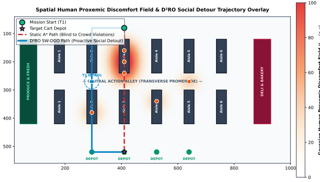
Fig. 1: Continuous 2D Gaussian Discomfort Field H_{\text{prox}}(x, y) heatmap and trajectory overlay comparing Static A^* (blind path through Aisle 3 crowd) against D 2 RO proactive social detour along Action Alley.
