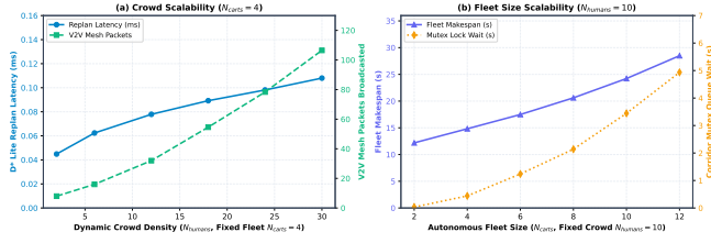
Fig. 10: Decoupled fleet scalability evaluations: (a) Incremental D* Lite replanning latency and V2V mesh broadcast packets vs. dynamic crowd density ( N_{\text{humans}} \in [2..30] , fixed fleet N = 4 ); (b) Fleet makespan and single-file corridor mutex queueing wait time vs. autonomous fleet size ( N_{\text{carts}} \in [2..12] , fixed crowd N = 10 ).
