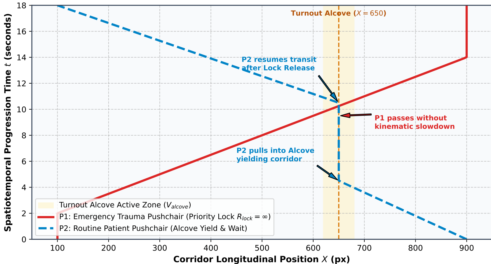
Figure 9: Spatiotemporal Time-Space Trajectory Diagram of Turnout Alcove Resolution
