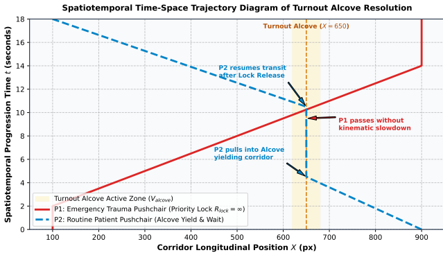
Fig. 5: Spatiotemporal time-space trajectory diagram of Turnout Alcove resolution: Emergency Pushchair P_1 maintains full velocity under priority lock R_{\text{lock}} = \infty , while routine Pushchair P_2 yields inside the alcove bay.
