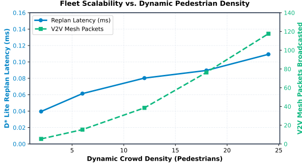
Fig. 10: Fleet scalability curves showing sub-linear D* Lite vertex repair latency and V2V mesh packets as crowd density increases from 2 to 24 pedestrians.
